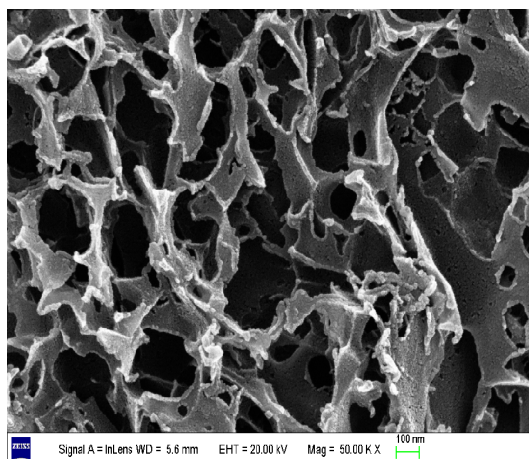
Figure S1. SEM image of BHPC-850 (Scale bar represents 100 nm)
