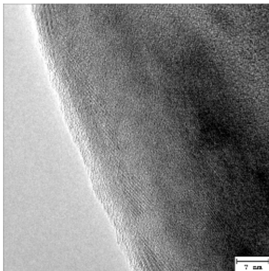
Figure S2. HRTEM image of BHPC-850
