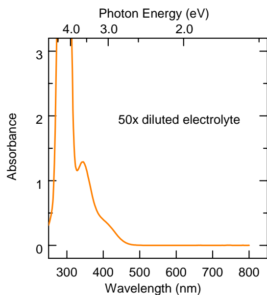
Fig. 2S. The absorbance spectra for CH 3 CN solution that contained 20 mM LiClO 4 , 0.4 mM Me 10 CoCp 2 + and 0.04 mM Me 10 CoCp 2 , which was diluted with CH 3 CN by a factor of 50 relative to the solution used in the spectral response measurements.
