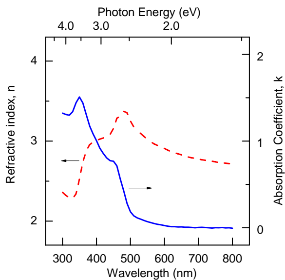
Fig. 1S. Optical constants of Cu 2 O substrates measured by spectroscopic ellipsometry in the spectra range of interest.
