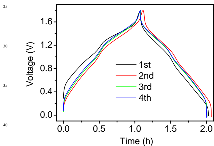
45 Fig. S2. Charge and discharge curve of activated carbon//porous \text{LiMn}_2\text{O}_4 in the initial 4 cycles at the current density of 100 \text{ mA g}^{-1} .
