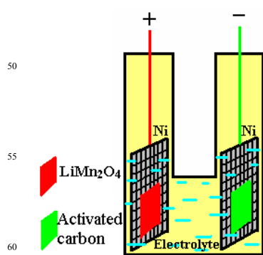
Fig. S3 The schematic figure of the two-electrode cell.
