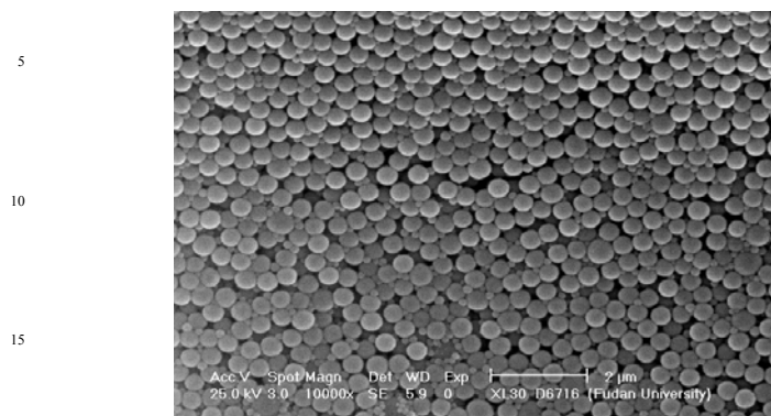
20 Fig. S1. Scanning electron micrograph of the PS template.
