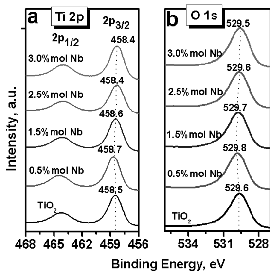
Figure S1. XPS spectra of the (a) Ti 2p and (b) O 1s core level of undoped and Nb-doped TiO 2
