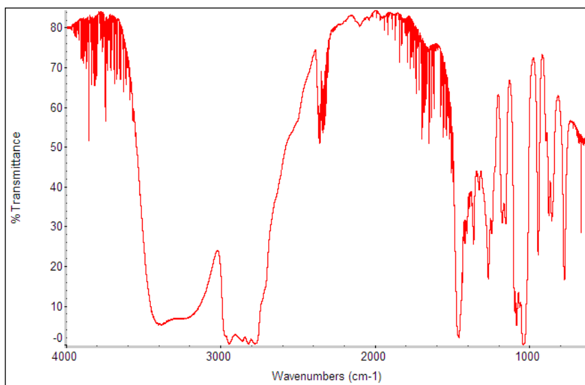
Figure S3. IR of DMEA on NaCl plates.
