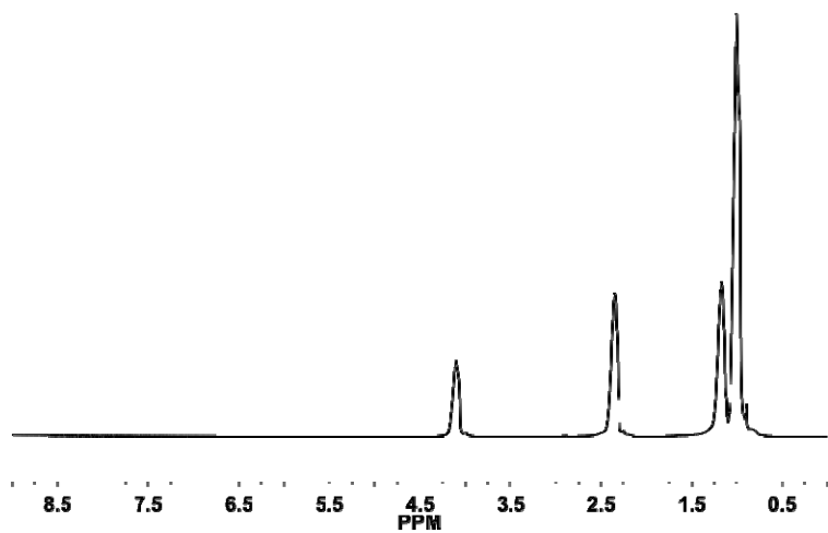
Figure S1. 1 H NMR spectrum of neat DMEA
