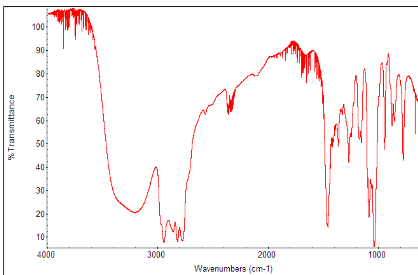
Figure S4. IR of DMEA + H 2 S on NaCl plates
