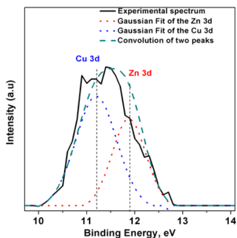
Figure S1. UPS spectra in the vicinity of the Zn 3d and Cu 3d core-level emissions on an expanded scale. The spectra were taken at etch level 15 over an etch time of 1500 s. The peak fitting and deconvolution were performed on the spectrum interval of 10 to 12 eV. The fitting was done after a Shirley-type background subtraction. The peak is decomposed into two Gaussian functions.
