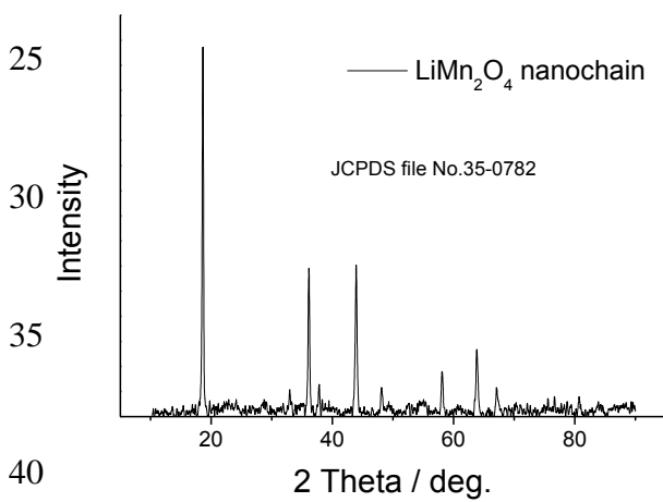
Fig. S2. XRD of LiMn 2 O 4 nanochain.
