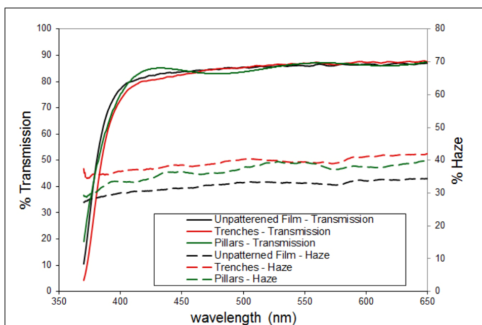
Fig. S1 Transmission and haze measurements on unpatterned films, trenches and pillars.
