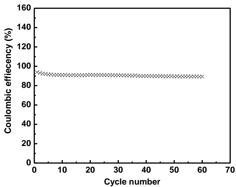
Figure S2. Coulombic efficiency of a Na-S battery at 150°C.
