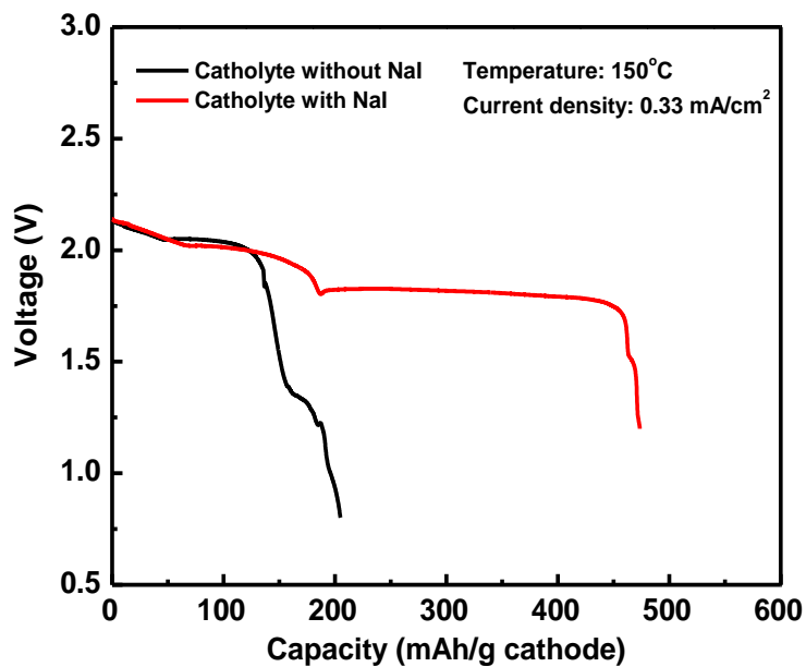
Figure S1. Initial discharge curves of Na-S batteries with and without addition of NaI into the tetraglyme 30 catholyte.
