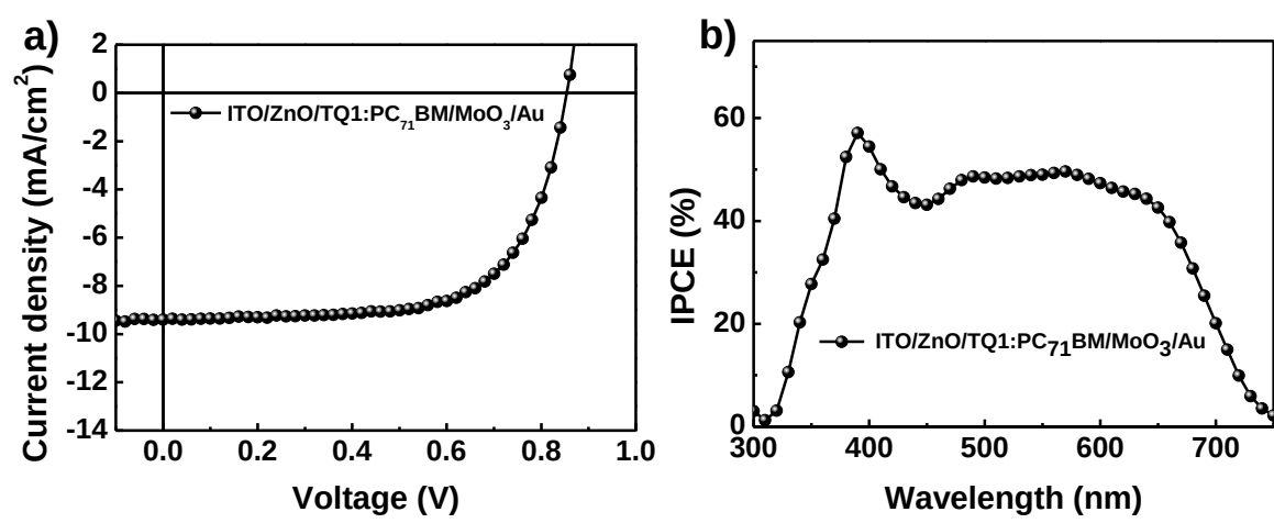
Figure S3. (a) J - V characteristics and (b) IPCE of the inverted TQ1:PC 71 BM PSCs using Au. J SC = 9.40 mA/cm 2 , V OC = 0.85 V, FF = 0.67, PCE = 5.35%.
