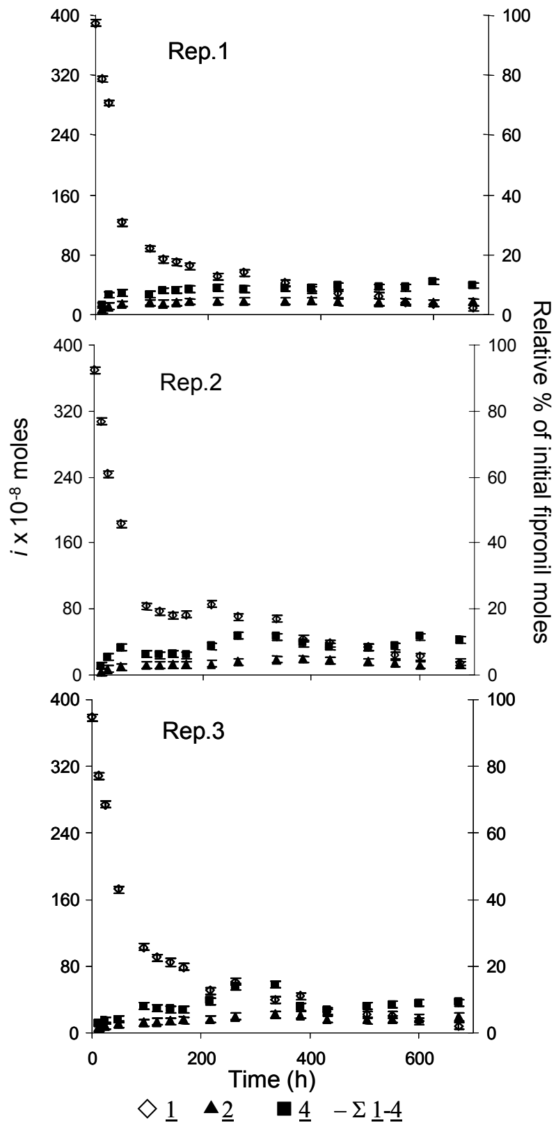
Sup. Figure 6. Aqueous product distribution of fipronil in estuarine mesocosms over the timescale of the experiment.
