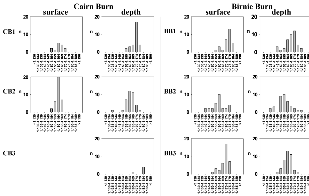
Fig.A11 Histograms of ^{206}\text{Pb}/^{207}\text{Pb} ratio (typical error \pm 0.004 ) for soil porewaters collected from Prenart samplers located near each of the stream water sampling sites during the period October 2001-August 2003.
