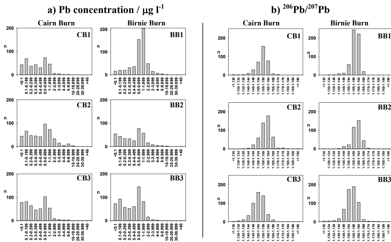
Fig. A12 Histograms of a) Pb concentration and b) ^{206}\text{Pb}/^{207}\text{Pb} ratio for stream water at CB1-3 and BB1-3 during the period October 2001-August 2003.
