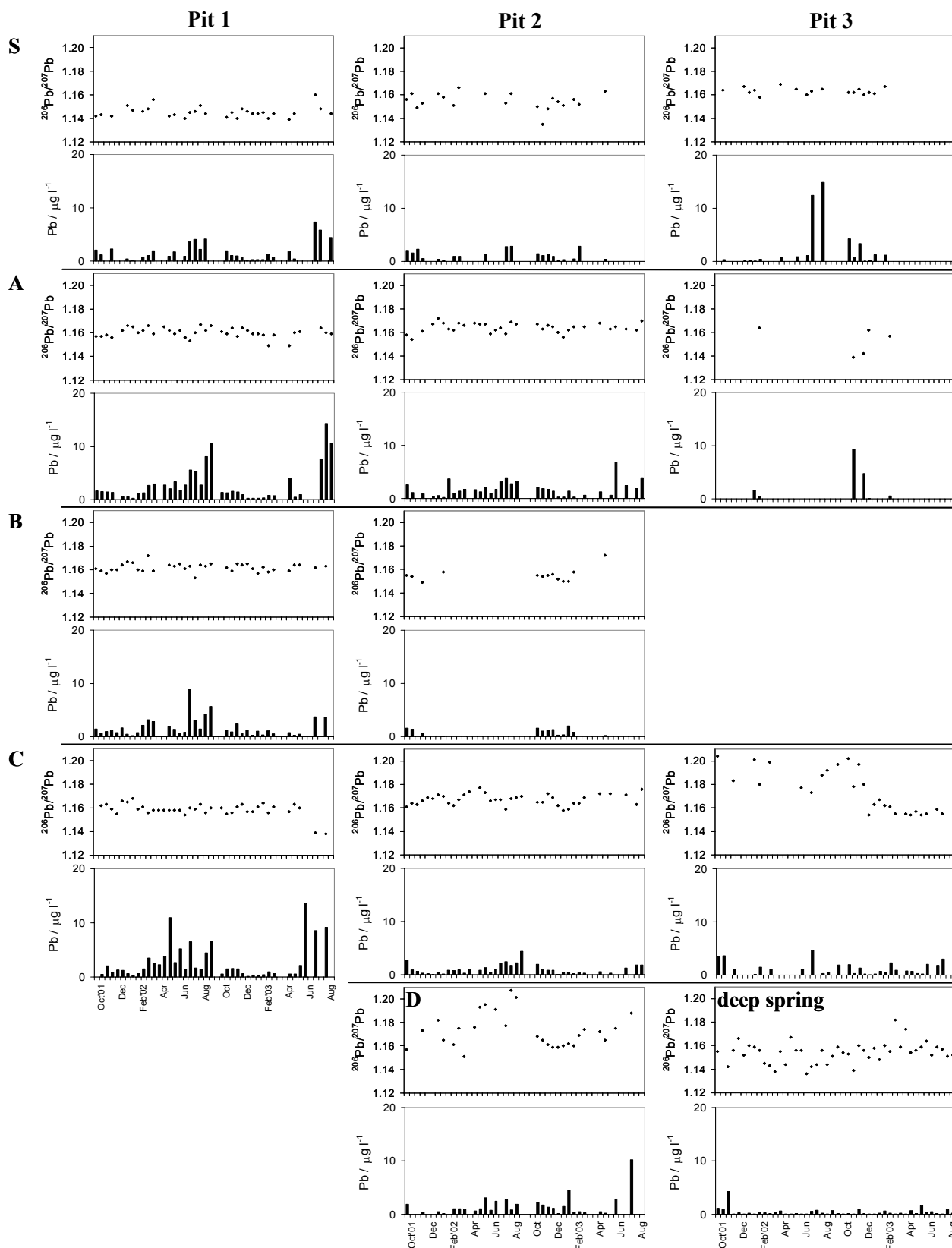
Fig. A5 ^{206}\text{Pb}/^{207}\text{Pb} ratios (typical error \pm 0.004 ) and Pb concentrations for soil throughflow collected at two-weekly intervals from Pits 1-3 during the period October 2001-August 2003 at Glensaugh.
