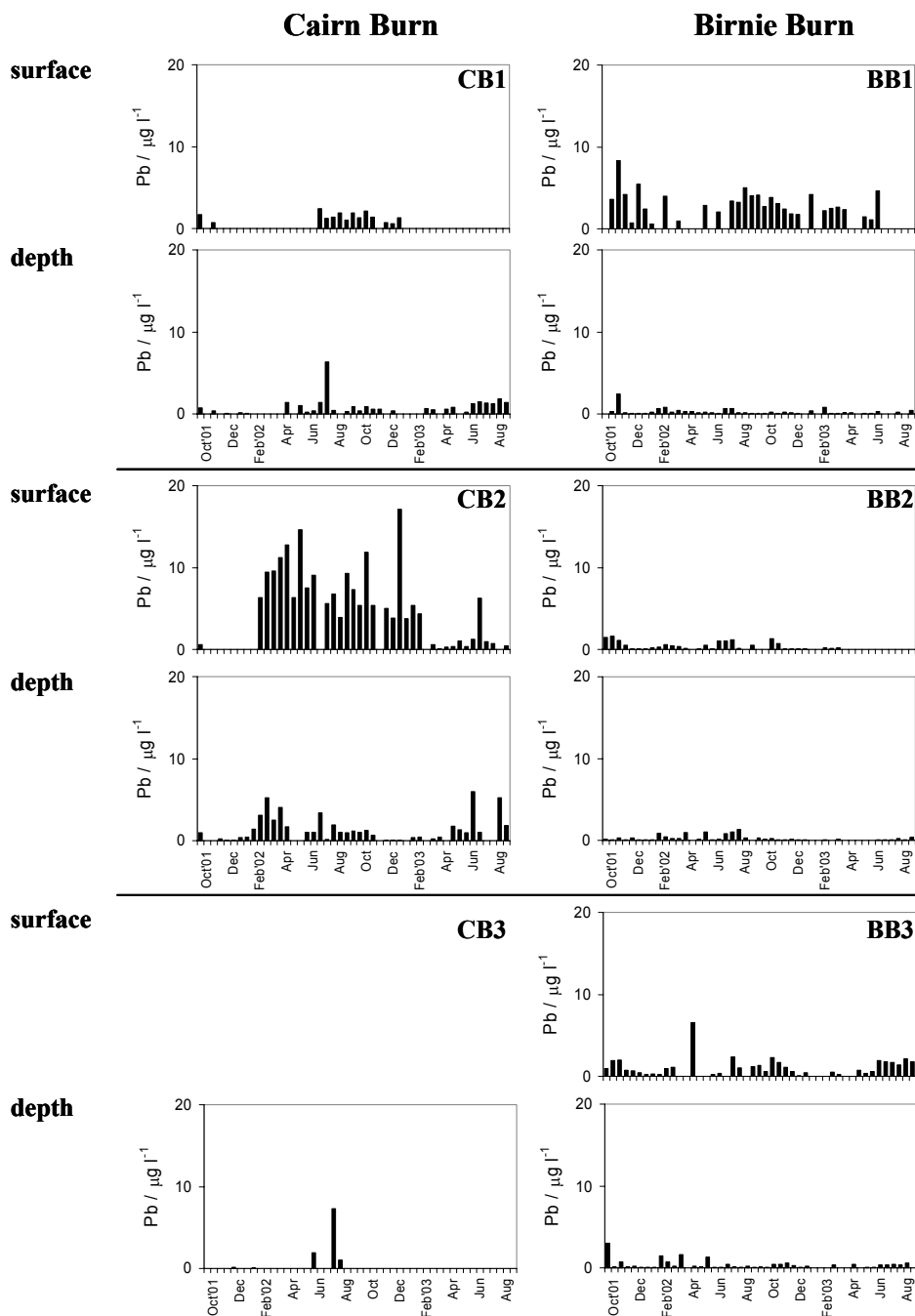
Fig. A9 Pb concentrations for soil porewaters collected at two-weekly intervals from Prenart samplers located near each of the stream sampling sites during the period October 2001-August 2003 at Glensaugh.
