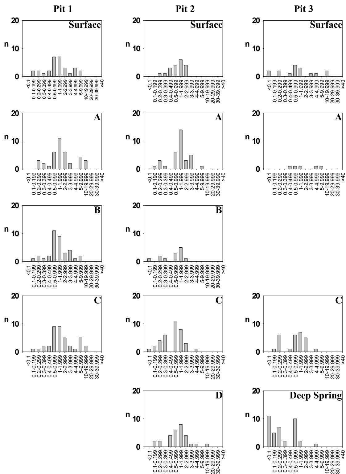
Fig. A6 Histograms of Pb concentration ( \mu\text{g l}^{-1} ) for soil throughflow at Pits 1, 2 and 3 during the period October 2001-August 2003.
