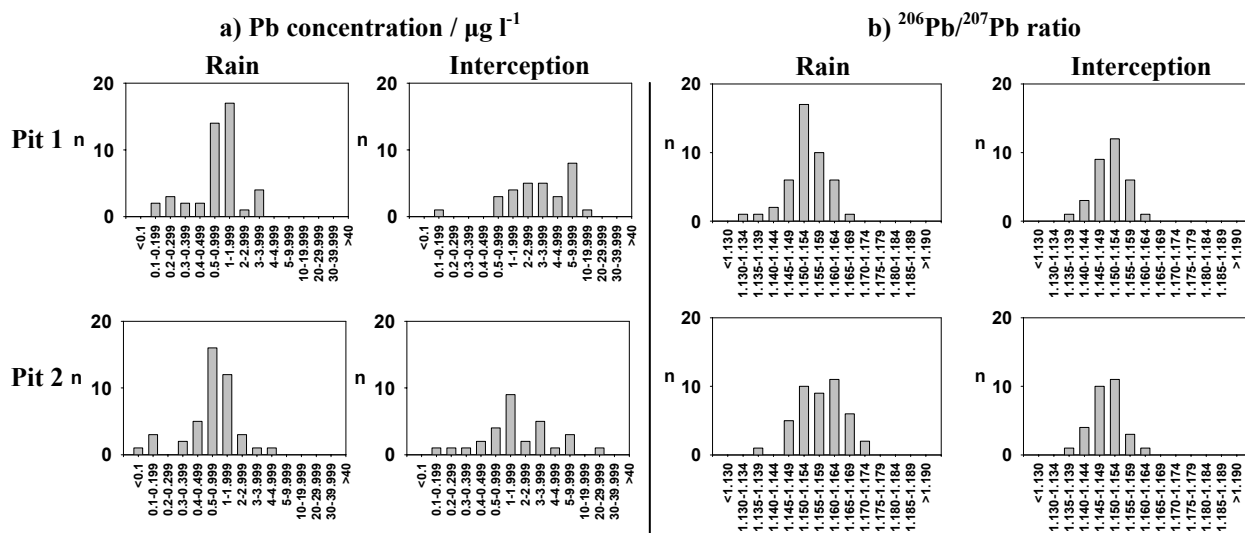
Fig. A1 Histograms of a) Pb concentration and b) ^{206}\text{Pb}/^{207}\text{Pb} ratio for rain water (October 2001-August 2003) and interception (May 2002-August 2003) at Pits 1 (n=44;43) and 2 (n=44;30).
