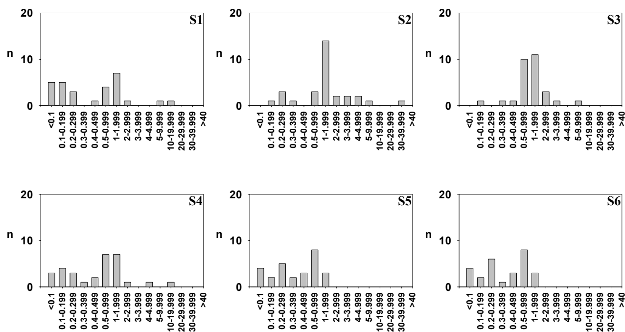
Fig. A3 Histograms of Pb concentration ( \mu\text{g l}^{-1} ) for spring flows S1-6 during the period May 2002-August 2003.
