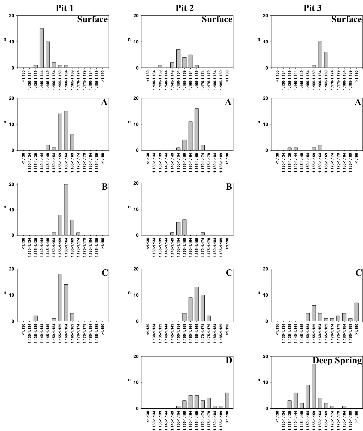
Fig. A7 Histograms of ^{206}\text{Pb}/^{207}\text{Pb} ratio for soil throughflow at Pits 1-3 during the period October 2001-August 2003.
