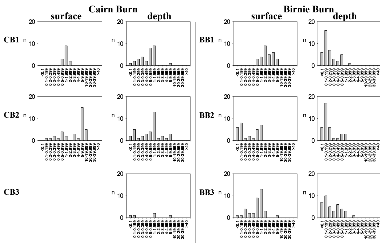
Fig. A10 Histograms of Pb concentration ( \mu\text{g l}^{-1} ) for soil porewaters collected from Prenart samplers located near each of the stream water sampling sites during the period October 2001-August 2003.
