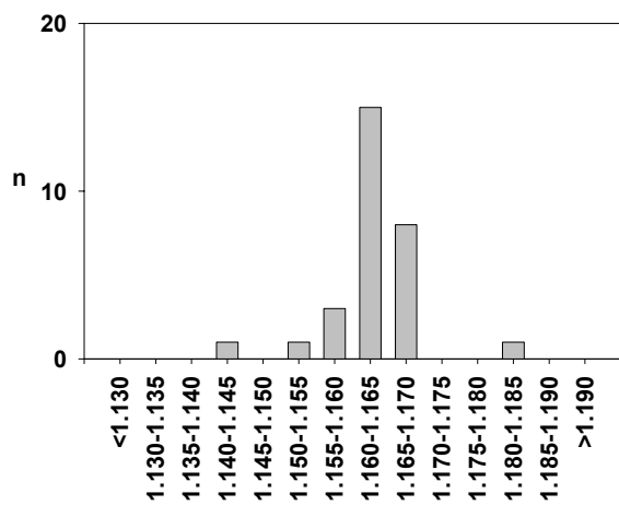
Fig. A14 ^{206}\text{Pb}/^{207}\text{Pb} ratio in stream waters at Glensaugh when Pb concentration was > 5 \mu\text{g l}^{-1} during the period October 2001-August 2003.
