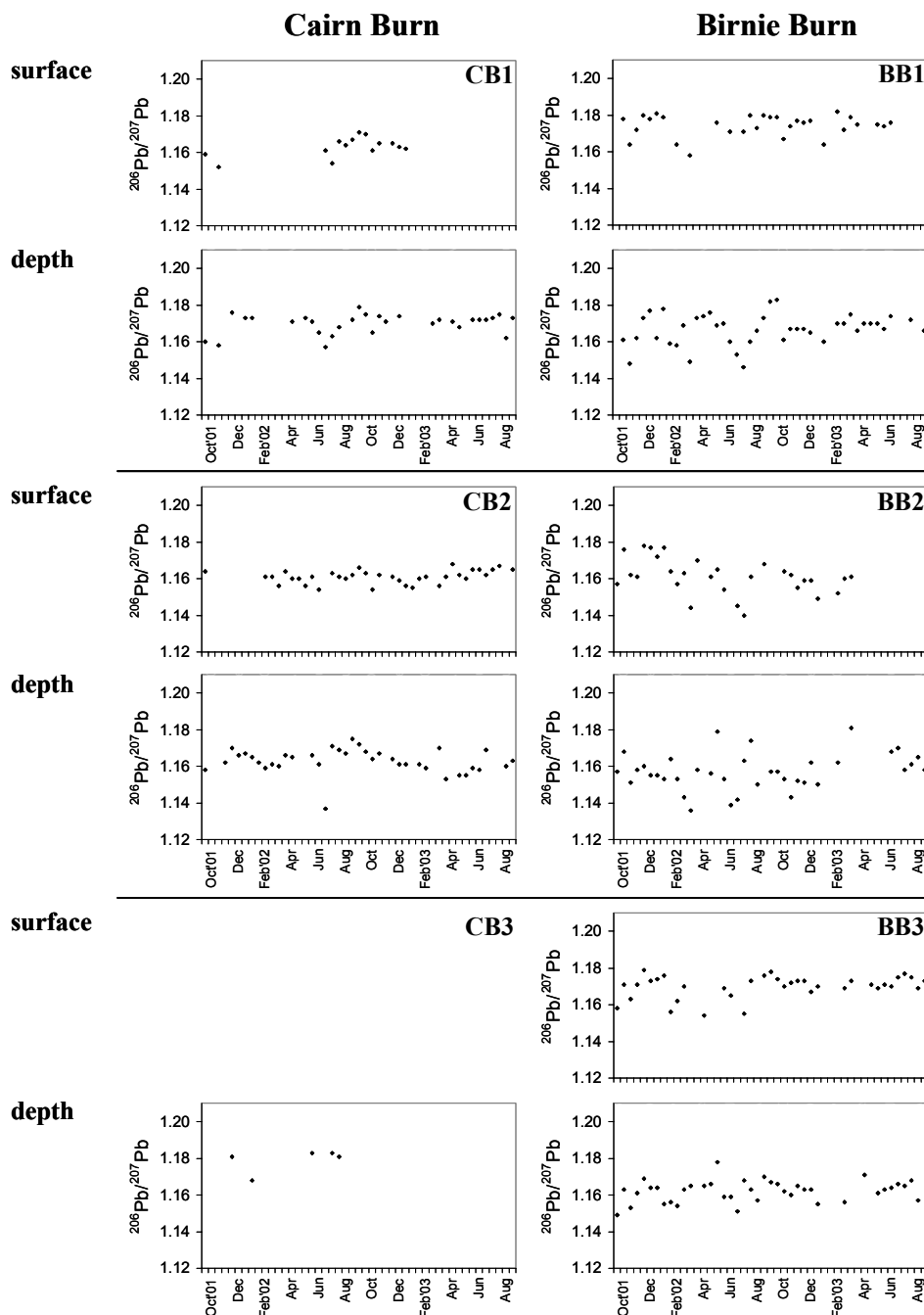
Fig. A8 ^{206}\text{Pb}/^{207}\text{Pb} ratios (typical error \pm 0.004 ) for soil porewaters collected at two-weekly intervals from Prenart samplers located near each of the stream sampling sites during the period October 2001-August 2003 at Glensaugh.
