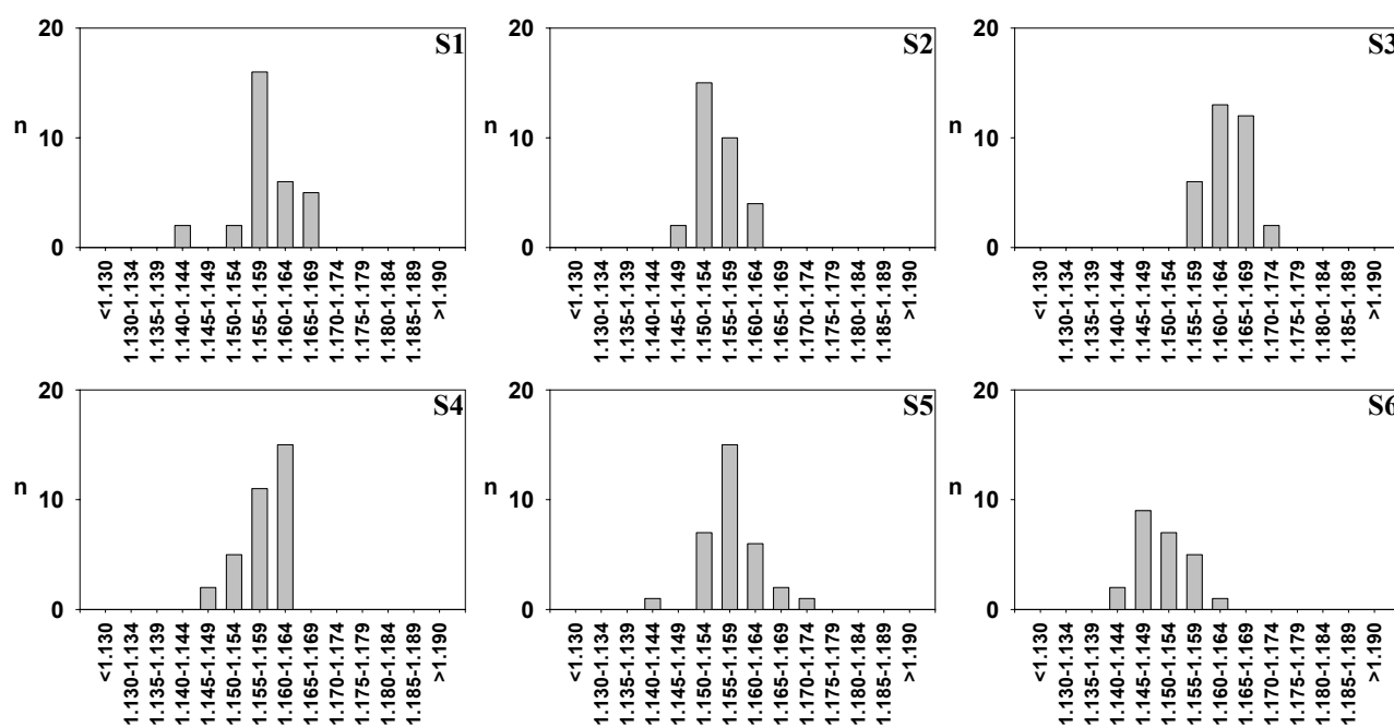
Fig. A4 Histograms of ^{206}\text{Pb}/^{207}\text{Pb} ratio for spring flows S1-6 during the period Oct 2001-Aug 2003.
