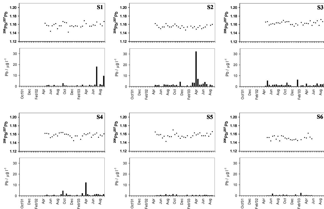
Fig. A2 ^{206}\text{Pb}/^{207}\text{Pb} ratios (typical error \pm 0.004 ) and Pb concentrations for spring flows S1-6 collected at two-weekly intervals during the period May 2002-August 2003 at Glensaugh.
