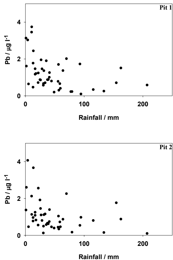
Fig. A13 Relationship between Pb concentration in rain water and rainfall (mm) at Glensaugh during the period October 2001-August 2003.
