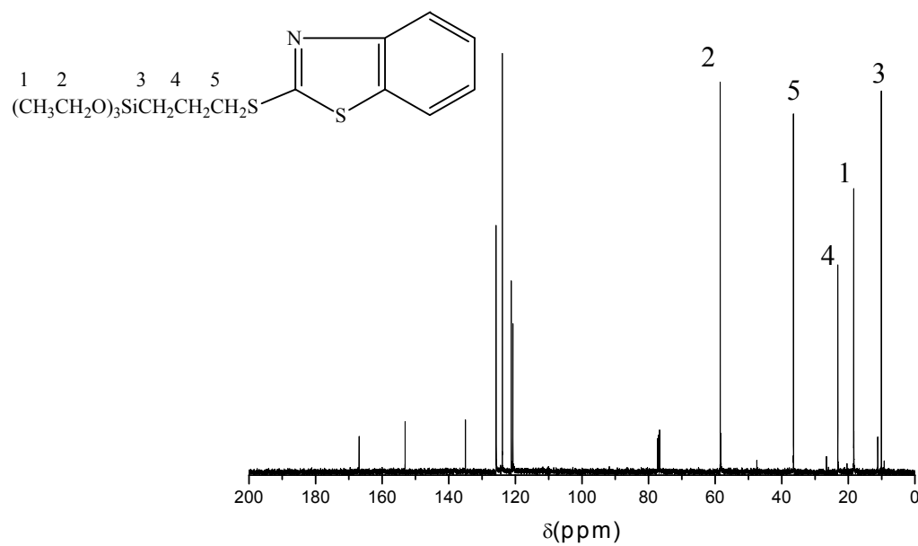
Fig. 3 ^{13}\text{C} NMR spectrum of mercaptobenzothiazole derivative in deuterated chloroform.
