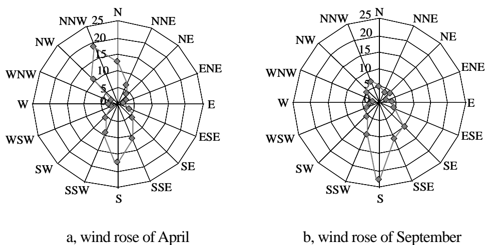
Fig. S1. Plot of April and September wind rose (Data from Dalian Environmental Monitoring Center)
