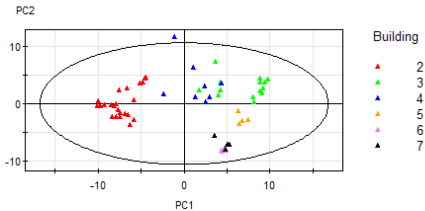
Figure S2 PCA score plot for the first two components of the model obtained from measurements with Chromosorb 106. Each triangle represents one measurement. The different colours represent different buildings.
