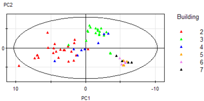
Figure S1 PCA score plot for the first two components of the model obtained from measurements with Carbo-pack B. Each triangle represents one measurement. The different colours represent different buildings.
