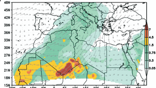
b) BSC/DREAM Dust Loading ( g/m^2 ) and 3000m Wind Oh forecast for 12z 29 JUN 06
