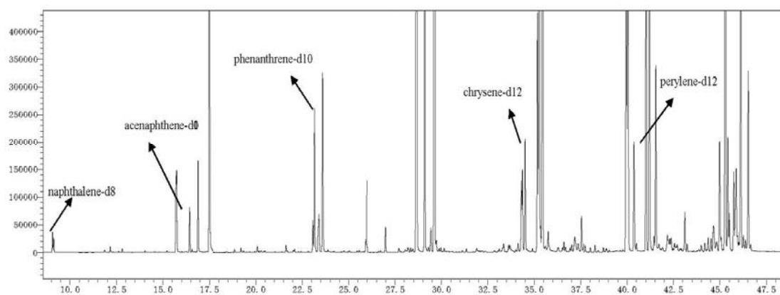
Fig S1. The gas chromatogram of one soil sample.
