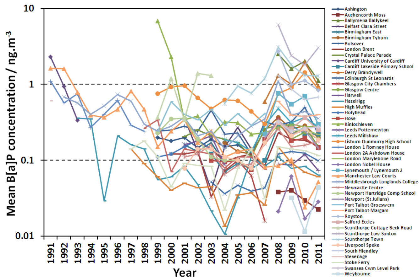
Figure ESI 1. Annual mean B[a]P concentration measured at all UK air quality network stations measuring PAHs since 1990. Only stations that have produced at least six individual monthly mean concentrations (or at least two quarterly mean concentrations) during a calendar year are included. The full dataset is available in Table 2.
