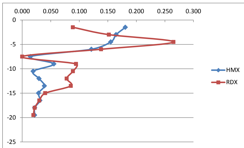
Figure S5: Background concentration profile of HMX and RDX in soil from bore hole 1 (T1) of the treatment plot
