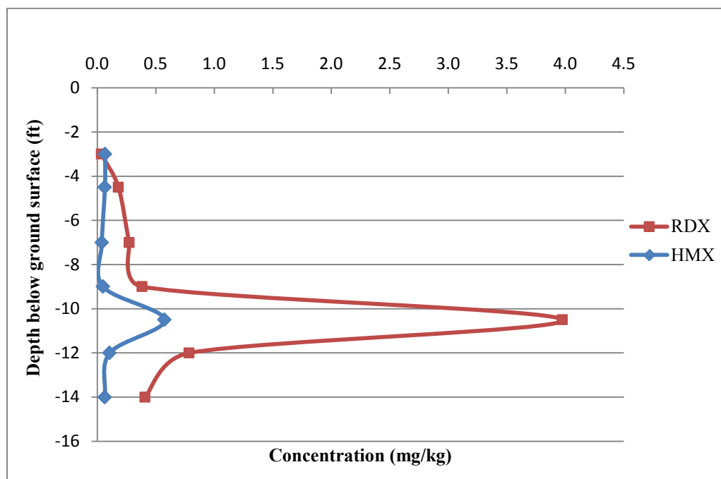
Figure S3: Background concentration profile of HMX and RDX in soil from bore hole 1 (C1) of the control plot
