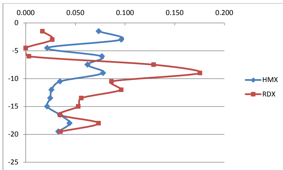
Figure S7: Background concentration profile of HMX and RDX in soil from bore hole 3 (T3) of the treatment plot
