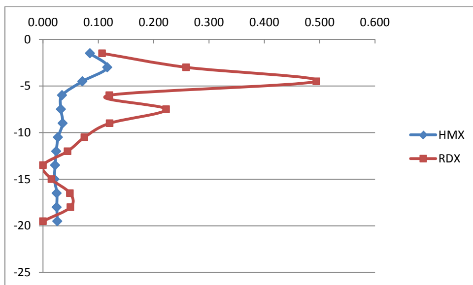
Figure S6: Background concentration profile of HMX and RDX in soil from bore hole 2 (T2) of the treatment plot
