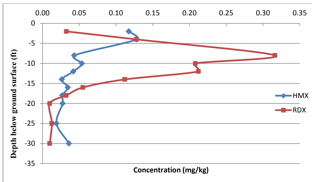
Figure S4: Background concentration profile of HMX and RDX in soil from bore hole 3 (C3) of the control plot
