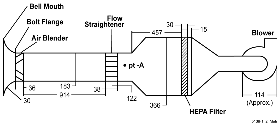
FIGURE S2. Schematic of wind tunnel with measurement in centimeters. (Adapted from Figure 1 of Cheng et al.)
