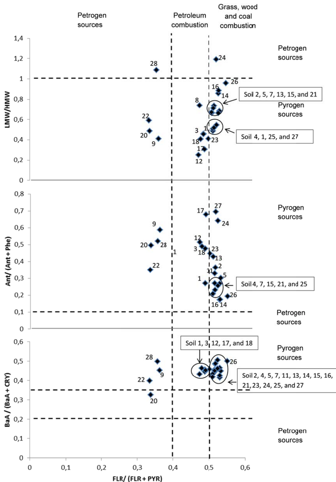
Figure S1 Cross plots of LMW to HMW (LMW/HMW), anthracene to the sum of anthracene and phenanthrene ( \text{Ant}/(\text{Ant} + \text{Phe}) ), and benz[a]anthracene to the sum of benz[a]anthracene and chrysene ( \text{BaA}/(\text{BaA} + \text{CRY}) ) against fluoranthene to the sum of fluoranthene and pyrene ( \text{FLR}/(\text{FLR} + \text{PYR}) ). Soils samples are labeled by numbers (see Table S2 for specification).
