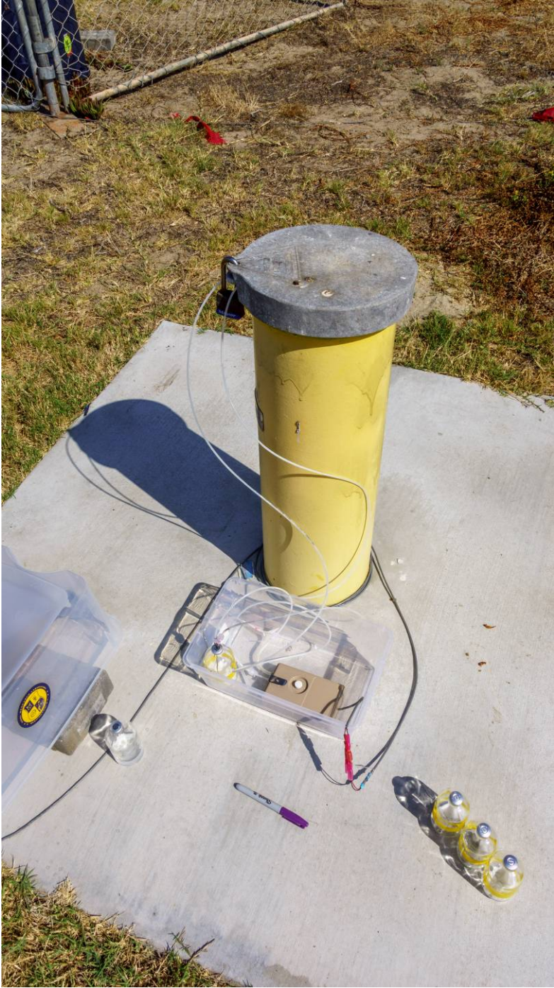
Pump deployment at well (traps are serum bottles)
