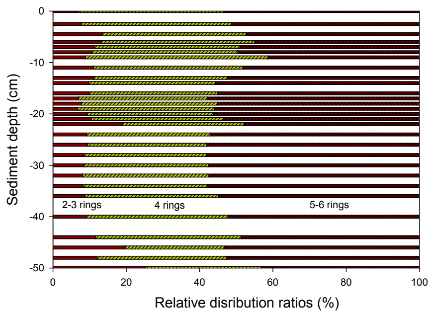
Fig. S1 The relative distribution profile of parent PAHs versus sediment depth
