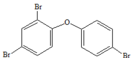
BDE 28
