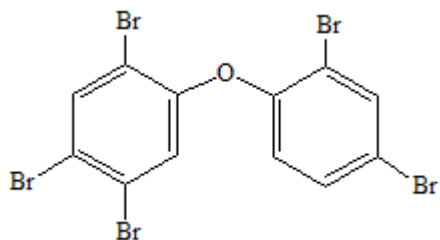
BDE 99
