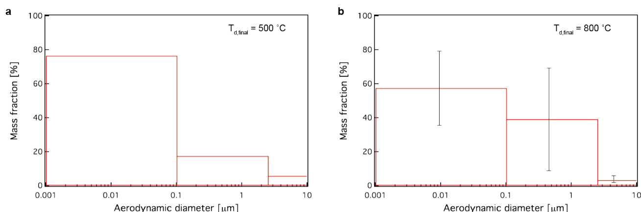
Figure S5. Particle size mass distributions for T_{d,final} = 500 (a) and 800 °C (b) as obtained by gravimetric analysis of the CCI stages.
