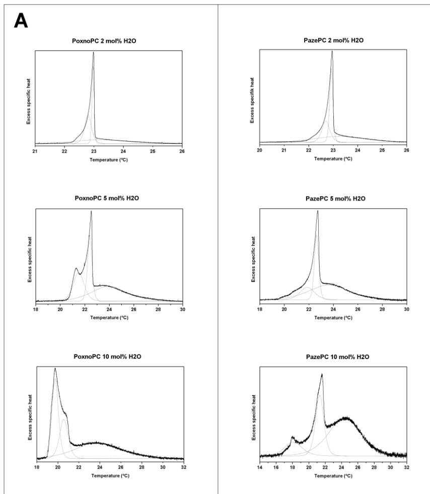
Supplementary Fig. 1A. Illustration of the results obtained in peak-fitting deconvolution analyses of the DSC thermograms of PoxnoPC- and PazePC-containing DMPC bilayers at different OxPI concentrations in 100 mM Tris/HCl (pH 7.4), 10 mM KCl, 140 mM NaCl, 0.5 mM EDTA using H 2 O as solvent.
