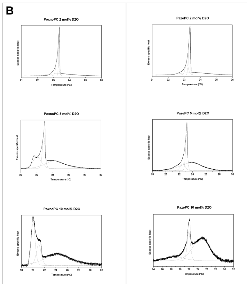
Supplementary Fig. 1B. Illustration of the results obtained in peak-fitting deconvolution analyses of the DSC thermograms of PoxnoPC- and PazePC-containing DMPC bilayers at different OxPI concentrations in 100 mM Tris/HCl (pH 7.4), 10 mM KCl, 140 mM NaCl, 0.5 mM EDTA using D 2 O as solvent.
