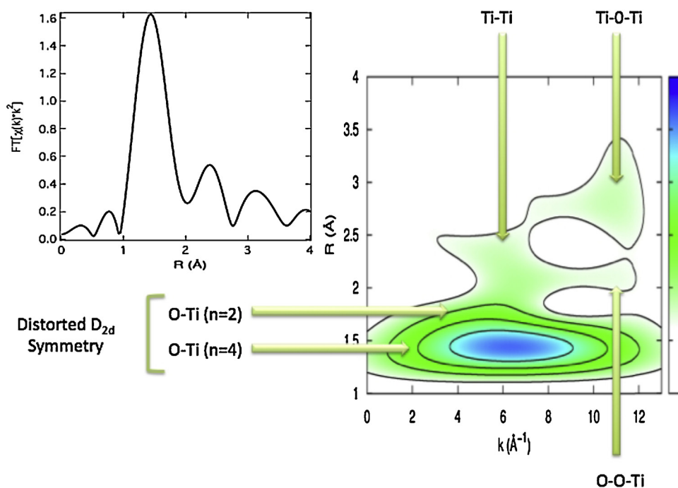
Fig. 18. The Fourier transform (upper left) and Wavelet transform of the EXAFS spectrum of anatase TiO 2 nanoparticles. The important scattering pathways are highlighted.
