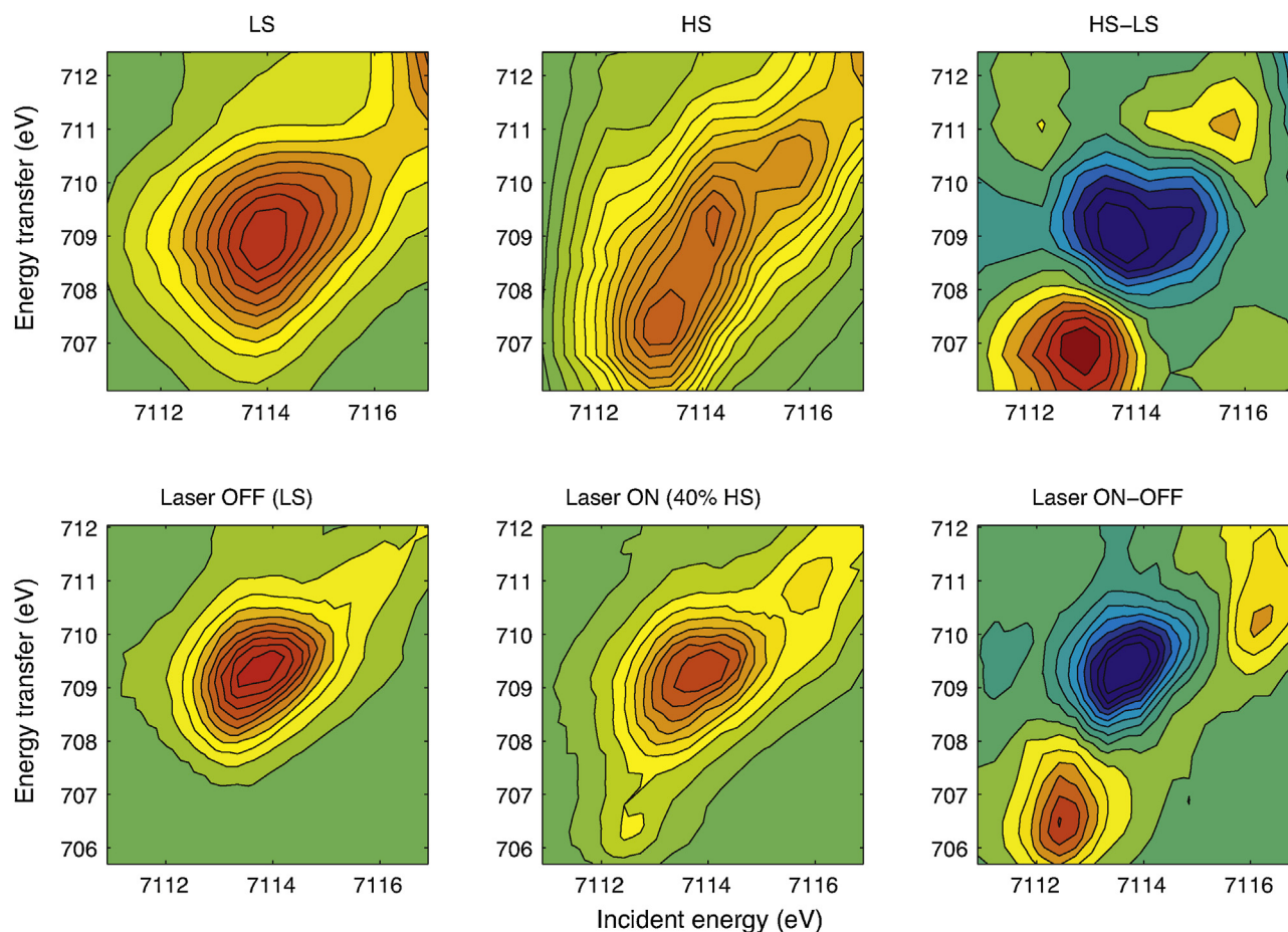
Fig. 13. Top: 1s2p 3/2 RIXS plane of solid [Fe(phen) 2 (NCS) 2 ] in its low-spin (left) and thermally-excited high-spin state (middle), with the difference between them shown on the right. Bottom: 1s2p 3/2 RIXS plane of aqueous [Fe(terpy) 2 ] 2+ before (left) and after laser excitation (middle), with the difference between them shown on the right. From Ref. [211].
