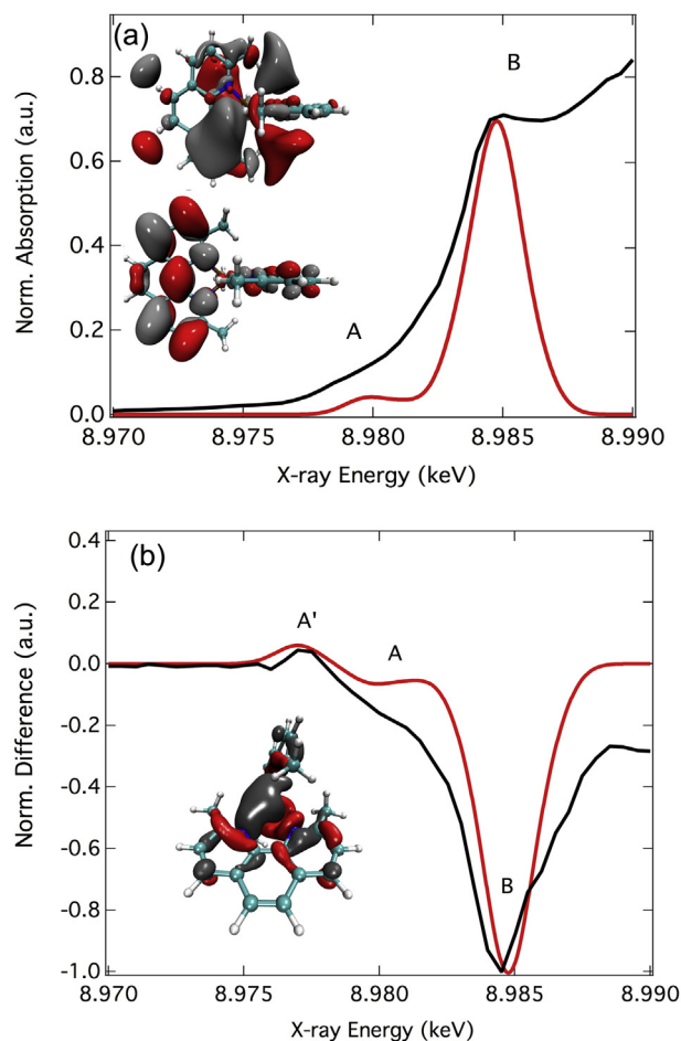
Fig. 15. (a) The pre-edge region of the spectrum and the oscillator strengths calculated using TDDFT with a 1.89 eV Lorentzian broadening. Inset is the molecular orbitals for the transition with the largest oscillator strengths for the two features. (b) The simulated pre-edge transient spectrum (red, ^3\text{MLCT} – ground-state) using TDDFT in comparison to the experimental transient (black). Inset is the molecular orbital for the transition with the largest oscillator strengths for the A'. Reproduced from Ref. [203].
