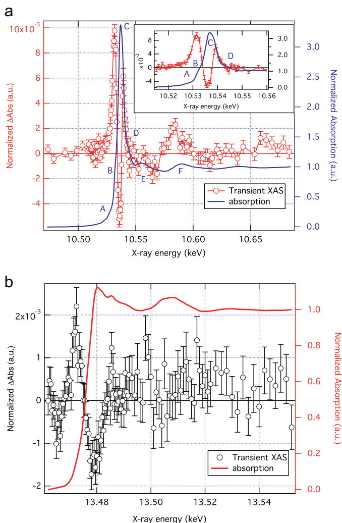
Fig. 10. Left: Normalised Re L 3 -edge transient XAS signal of a 30 mM solution of [ReBr(CO) 3 (bpy)] in N,N-dimethylformamide (red markers) measured 630 ps after excitation with 355 nm. The ground-state XAS is also shown for comparison (blue line) with features labelled A–F. Inset: zoom into the near-edge region to show the details of the transient XAS. Right: The corresponding normalised Br K-edge transient XAS signal measured on the same sample under the identical conditions. The ground-state XAS is also shown for comparison (red line). Figures reproduced from Ref. [201].
