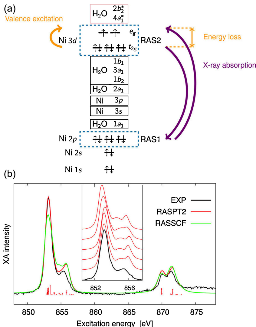
Fig. 17. (a) Schematic of the active space of the L_{2/3} -edge of aqueous NiCl_2 . The Ni\ 2p and Ni\ 3d are partitioned into two subspaces. RAS1 contains the Ni\ 2p orbitals with at most one hole, whereas RAS2 allows all possible electron permutations in the Ni\ 3d orbitals. Ligand-to-metal charge-transfer (LMCT) excitations can be accounted for by introducing ligand orbitals in RAS1 or RAS2. By introducing ligand orbitals in a third subspace RAS3 containing at most one electron, we can also model metal-to-ligand charge-transfer (MLCT) excitation. (b) Comparison between the experimental XAS of aqueous NiCl_2 and XAS calculated for Ni^{2+}(H_2O)_6 , with the RASSCF and RASPT2 methods. Reproduced from Ref. [52].
