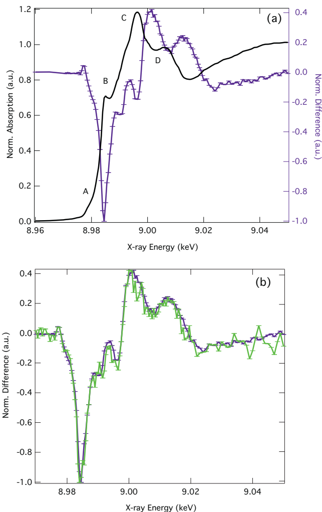
Fig. 11. (a) Static (black) and 50 ps transient Cu K-edge XANES spectra of [Cu(dmp) 2 ] + in acetonitrile (purple). Prominent features in the ground-state XAS are labelled A–D. (b) 50 ps transient Cu K-edge XANES spectra of [Cu(dmp) 2 ] + in acetonitrile (purple) and dichloromethane (green) [203]. In all cases the transient spectra have been normalised to the largest difference.
