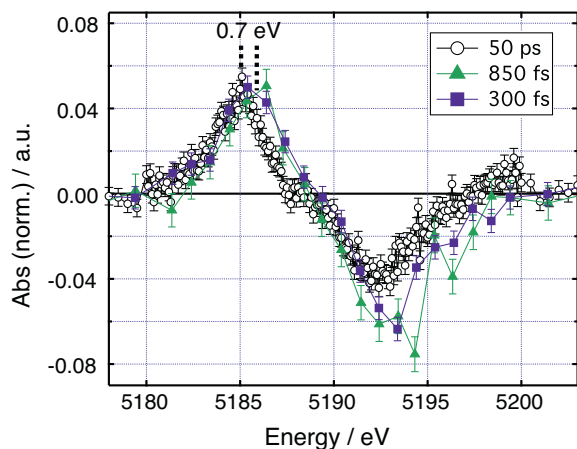
Fig. 14. Normalised transient L 1 -edge spectra of photoexcited aqueous iodide at 50 ps (black markers), 300 fs (purple markers), and 850 fs (green markers) time delays after excitation. The sub-picosecond transients were multiplied by a factor of 1.75 in order to match the value of the 50 ps transient at the maximum of the positive feature. Note the 0.7 eV shift to higher energies of the early time transient compared to the late time transient.
