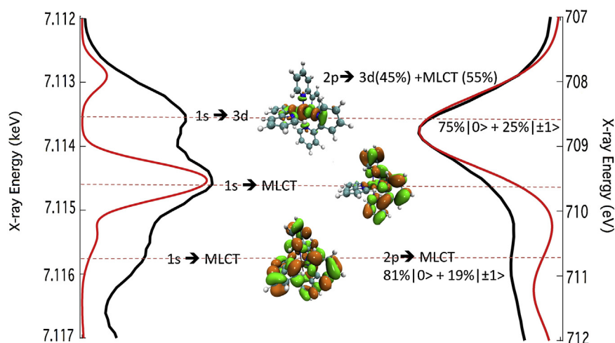
Fig. 16. A comparison of the features appearing in the pre-edge region of the Fe K-edge XAS (left) with the L 2/3 XAS edges (right) of [Fe(bpy) 3 ] 2+ . The important molecular orbital is shown alongside the corresponding transitions. The principal states and, in the case of the L 2/3 -edges, spin contributions are summarised with the respective transitions.
