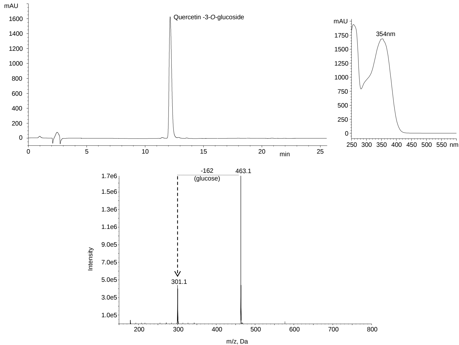
HPLC chromatogram recorded at 370 nm, UV spectrum and MS fragmentation of a standard of quercetin-3,O-glucoside
