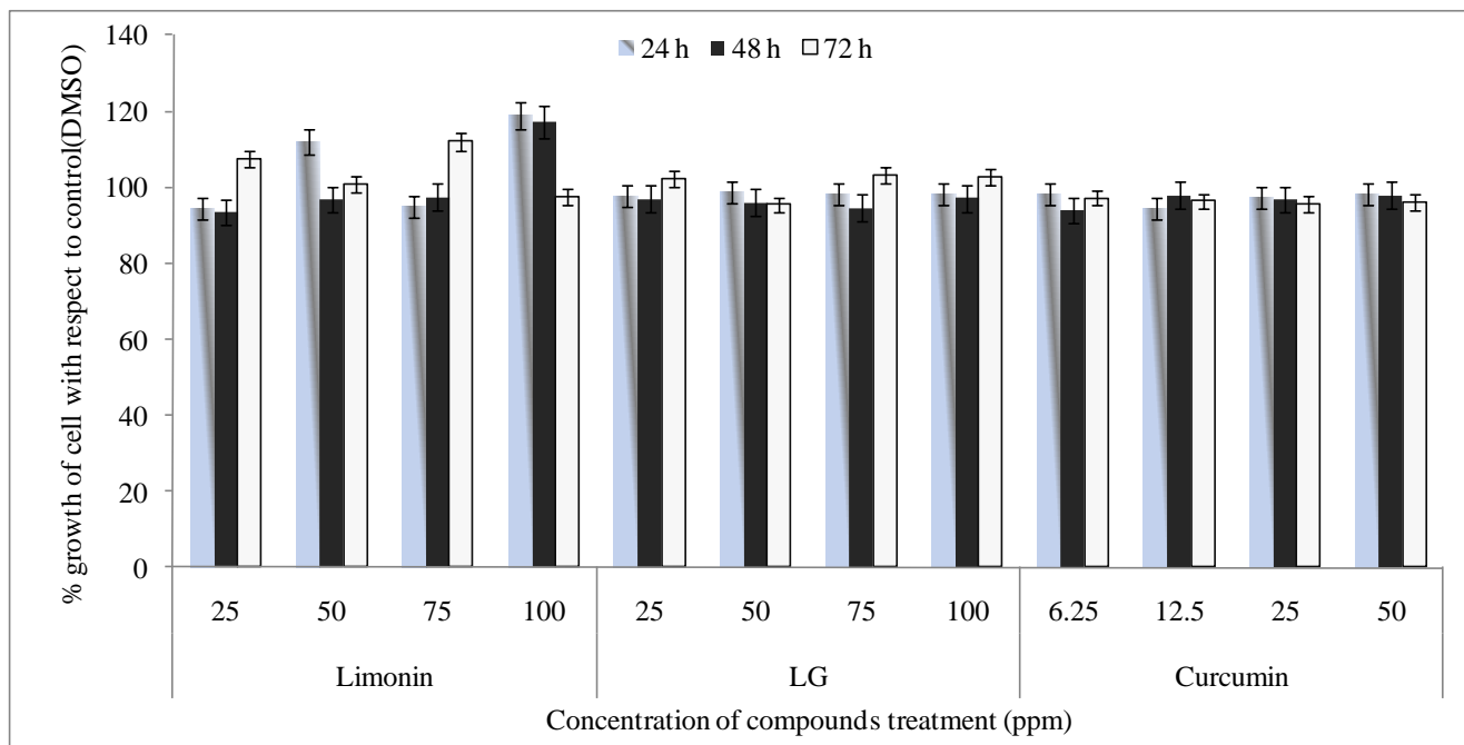
Fig. S1- Effect of limonin, LG and curcumin on proliferation of 112CoN cells measured by MTT assay. Cells were treated with the specified concentrations of compounds for 24, 48 and 72 h and amount of viable cells were spectrophotometrically estimated using MTT reagent. Results were expressed in % growth of cells compared to vehicle (DMSO) treated cells. There was no significance in differences in the % cell growth with samples treated compared to control (DMSO treated)
