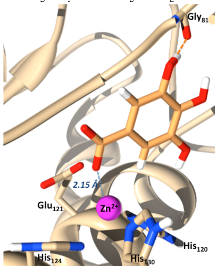
Figure S1. Most energetically favored binding mode of gallic acid in MMP-2.
