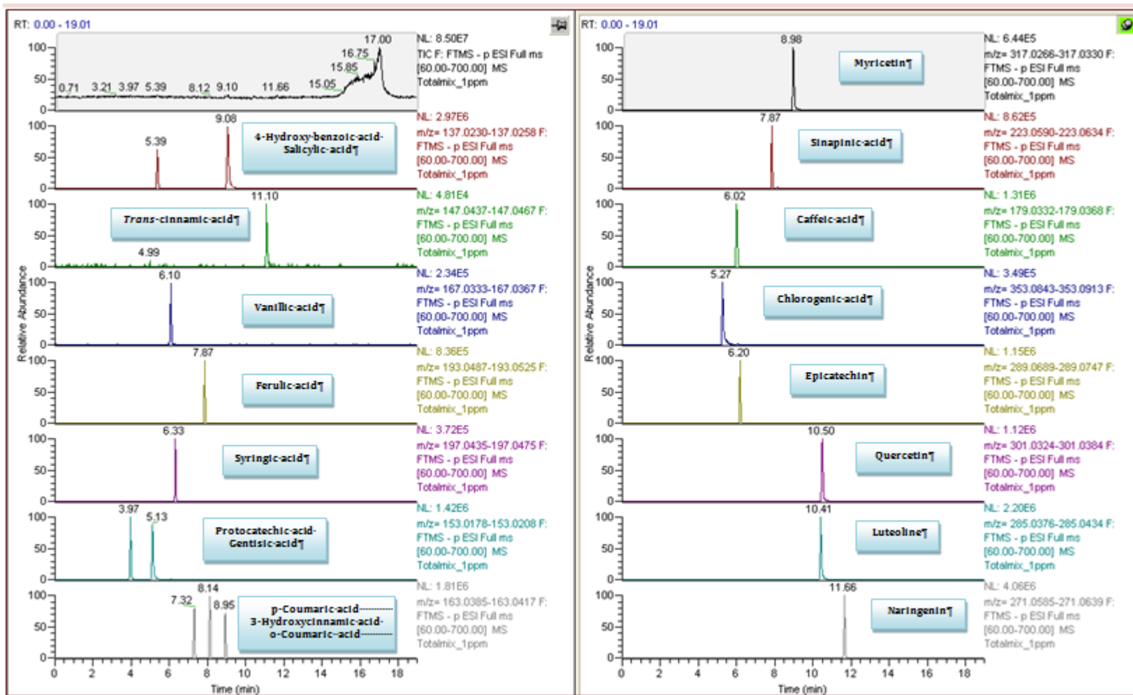
Figure S2. Total Ion Current and separated chromatograms of the standard mixture solution (1ppm) with the 19 standard phenolic compounds
