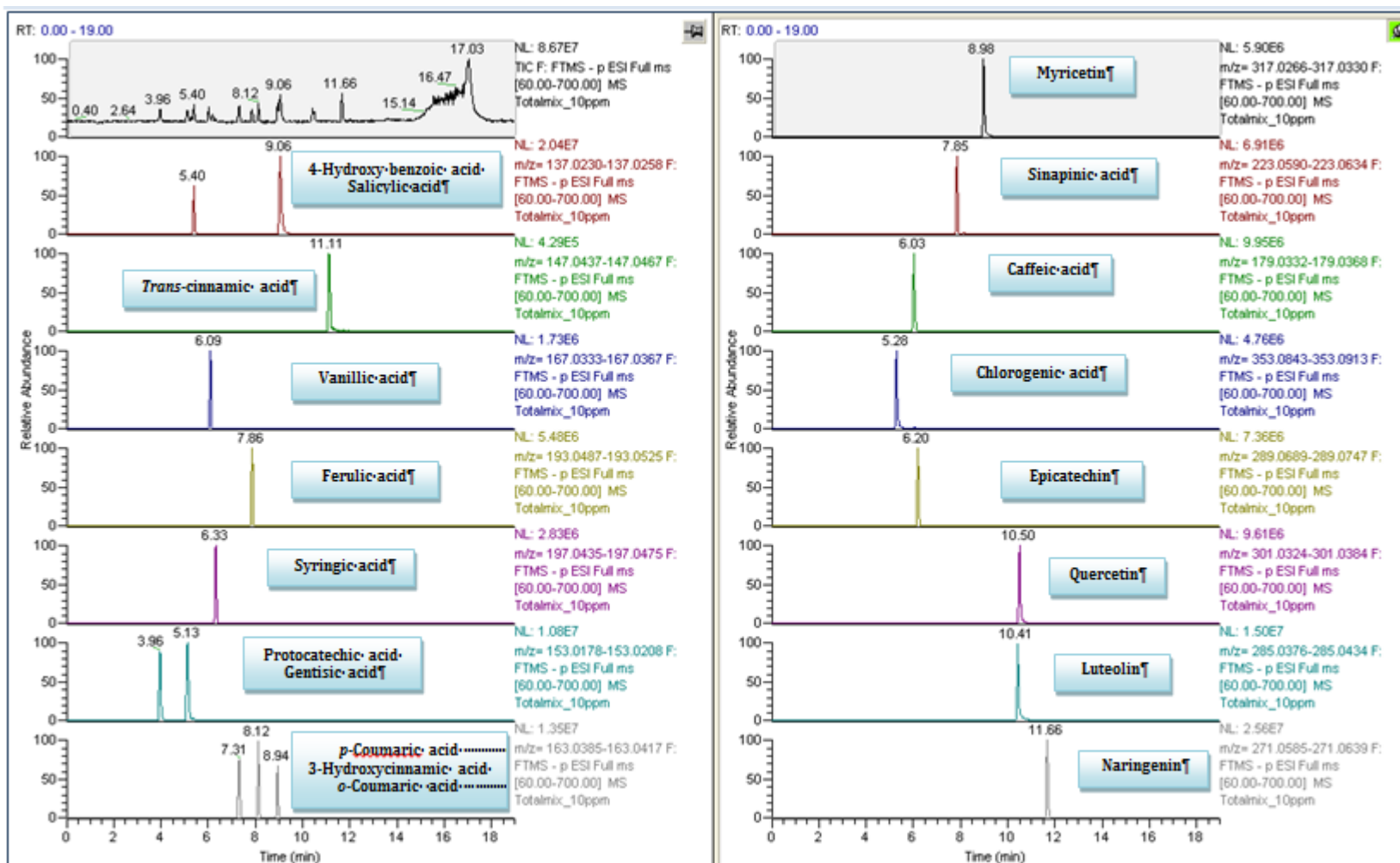
Figure S1. Total Ion Current and separated chromatograms of the standard mixture solution (10ppm) with the 19 standard phenolic compounds
