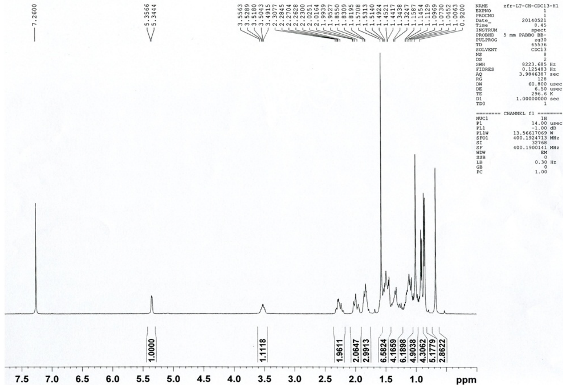
Supplementary Figure 1 NMR Spectra of cholesterol
