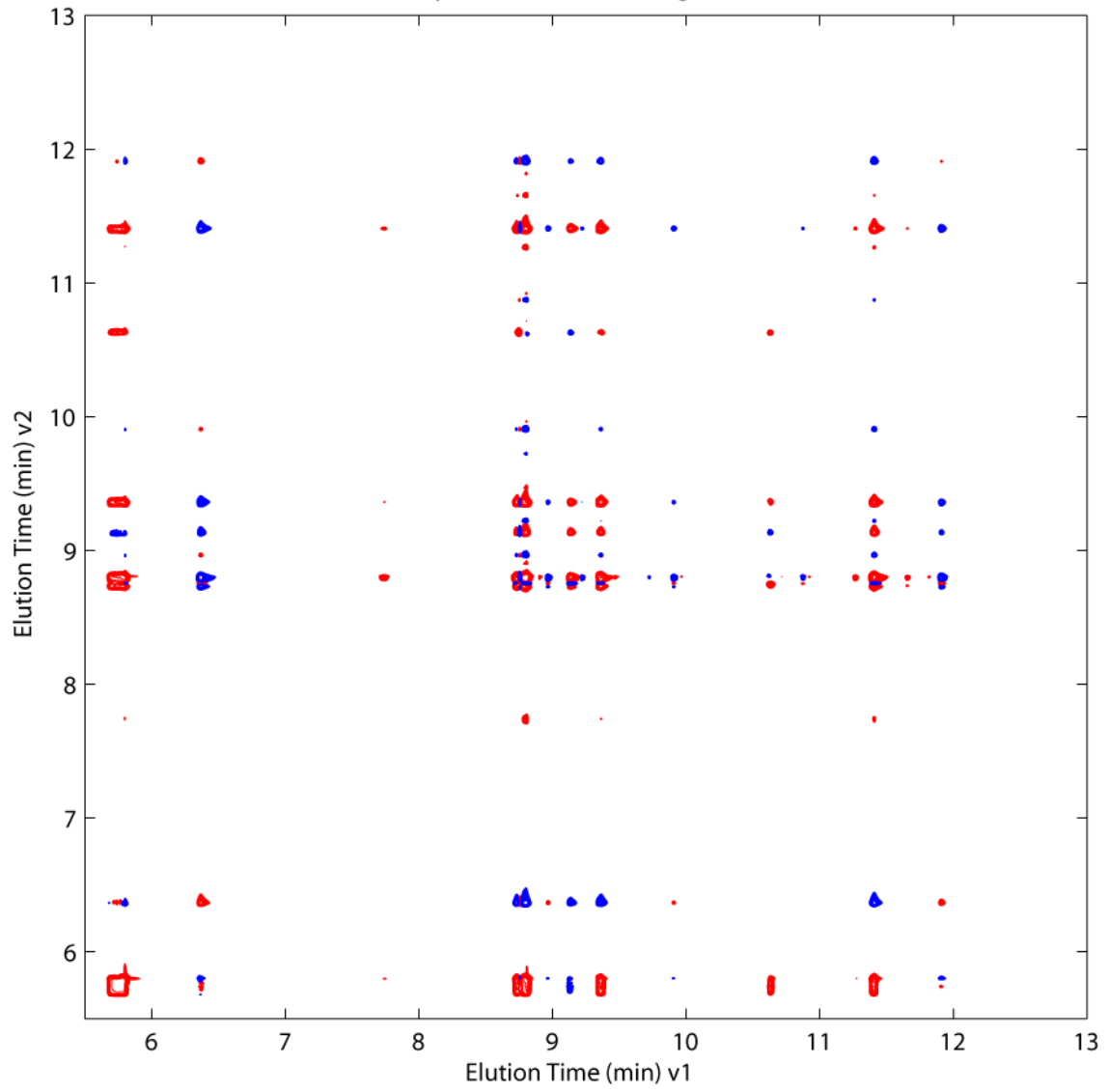
Synchronous Chromatogram
