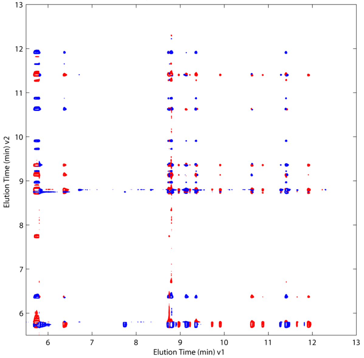
Asynchronous Chromatogram
