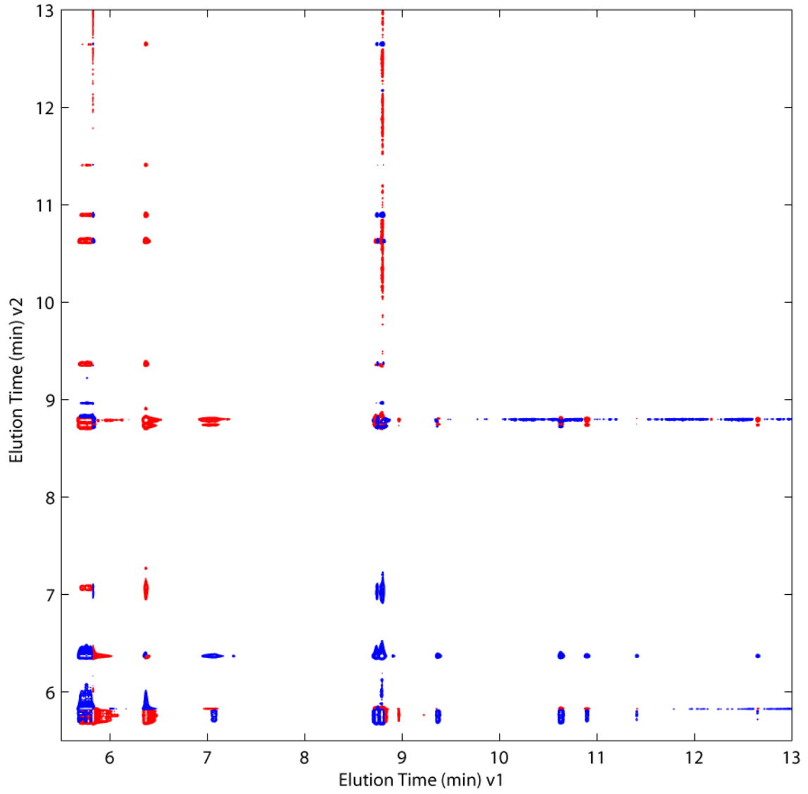
Asynchronous Chromatogram
