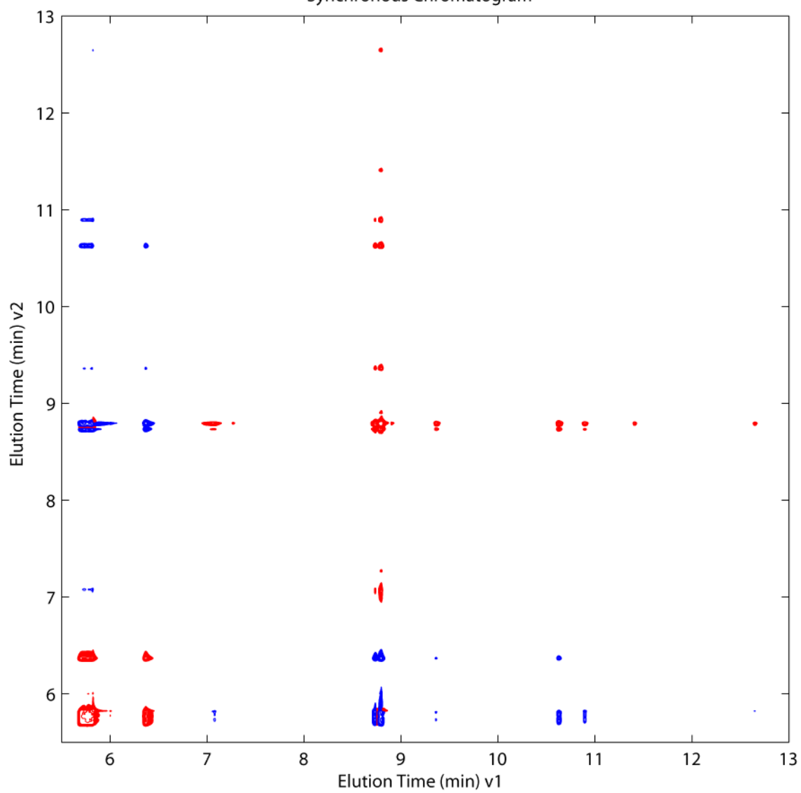
Synchronous Chromatogram
