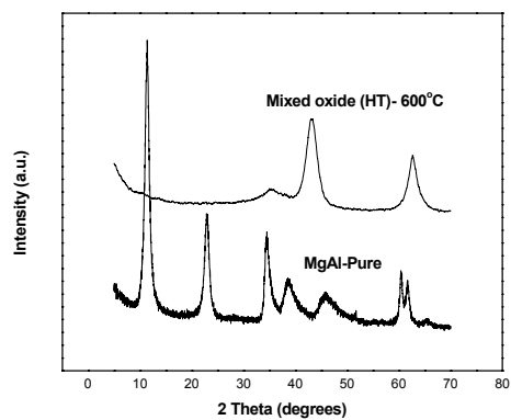
Fig 1S: PXRD pattern of MgAl-hydrotalcite and its calcined form ( mixed oxide) at 600°C
