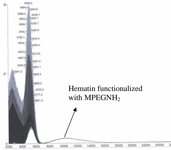
Figure 1: MALDI-TOF MS spectrum for the amidated hematin
