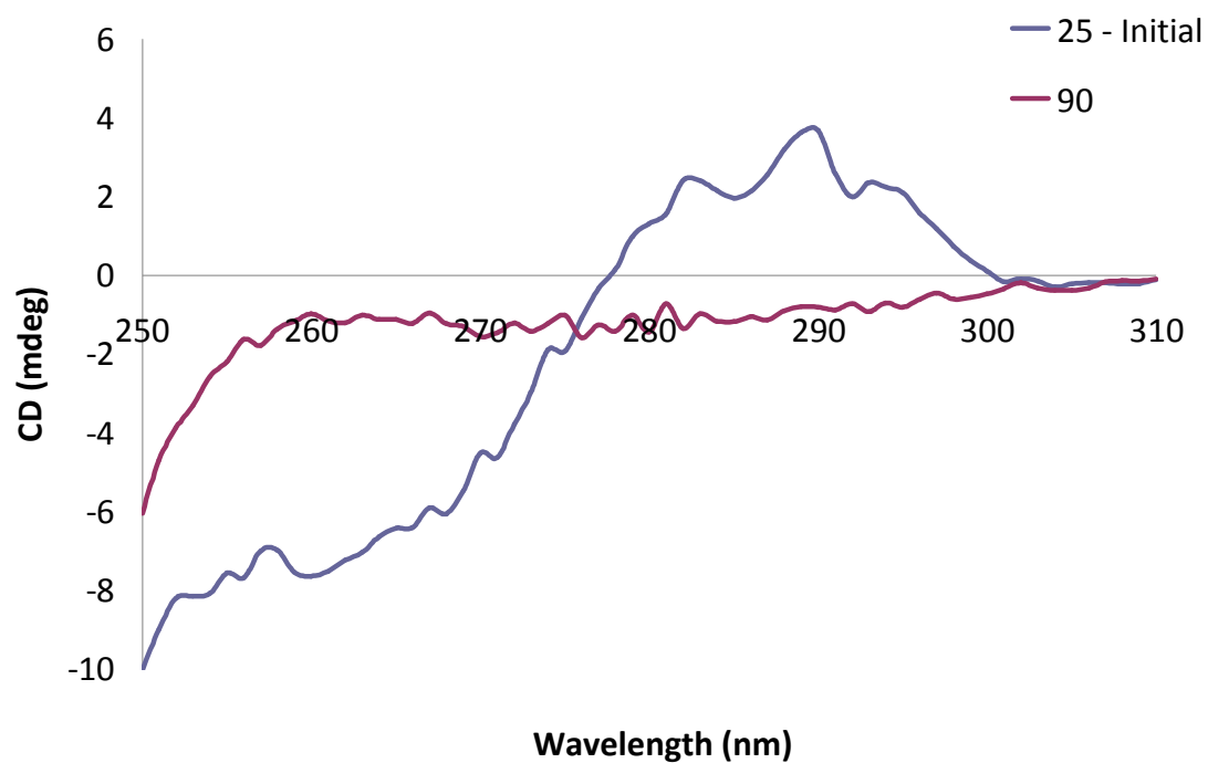
Supplementary Fig. A. Near UV CD spectrum of aqueous lysozyme ( 3.4 \times 10^{-4} mol.dm -3 ) in buffered water at 25 °C and 90 °C.
