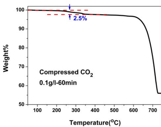
Figure S2. TGA curve of CaCO 3 particles obtained under control of 0.1g/l NaCMC after 60min reaction.
