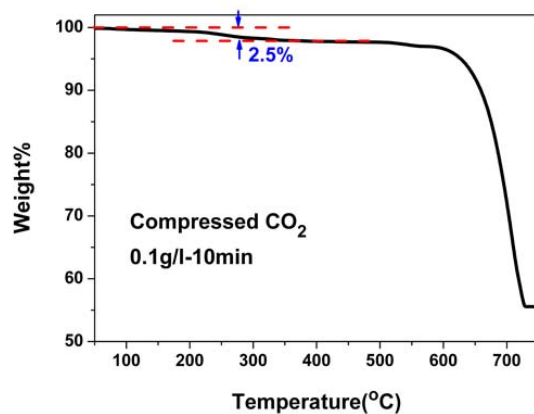
Figure S1. TGA curve of CaCO 3 particles obtained under control of 0.1g/l NaCMC after 10min reaction.
