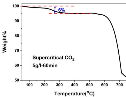
Figure S4 TGA curve of CaCO 3 particles obtained under control of 5g/l NaCMC after 60min reaction in scCO 2 .
