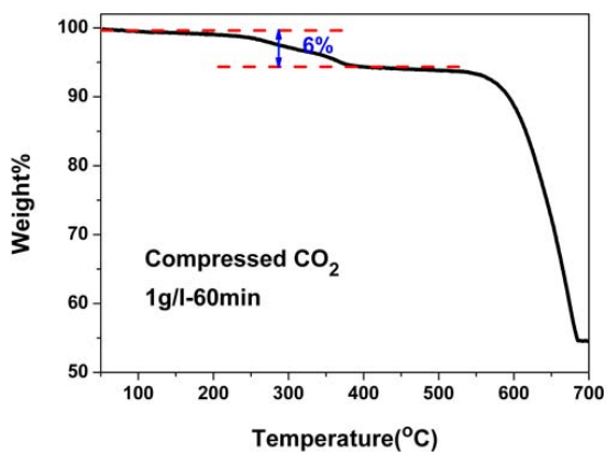
Figure S3. TGA curve of CaCO 3 particles obtained under control of 1g/l NaCMC after 60min reaction.
