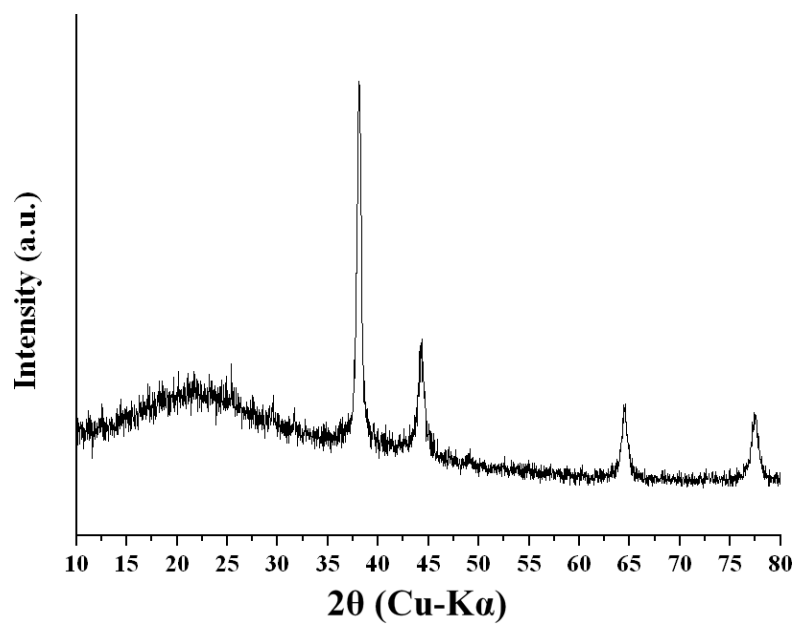
Supporting Information 1 (S1). XRD pattern of BT 800 -AuNPs.
