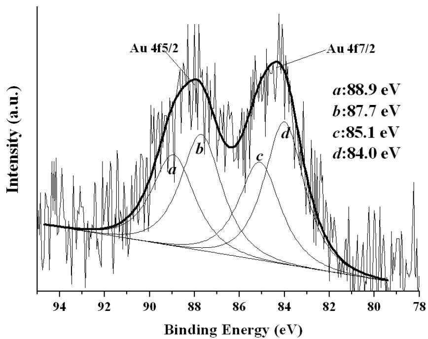
S2. XPS Au 4f spectra of BT 800 -AuNPs.
