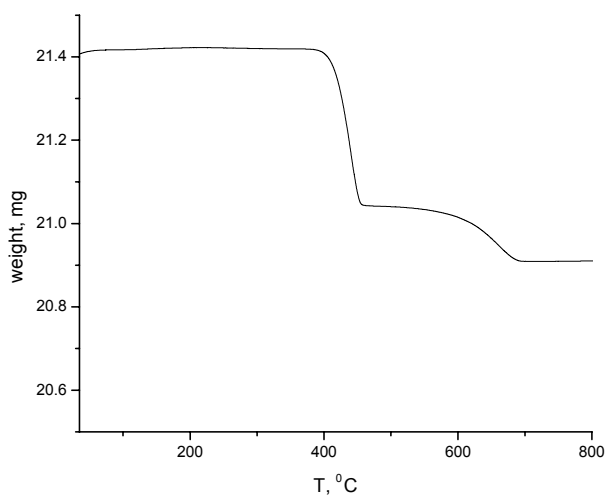
Figure S2. TG analysis of clinker B.
