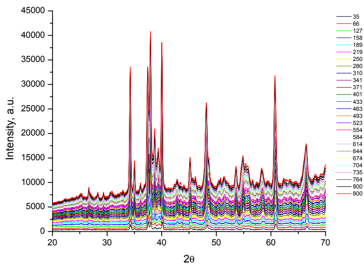
Figure S1. In-situ XRD measurements on clinker B-bio-glycerol mixture during calcination from room temperature to 800 °C.
