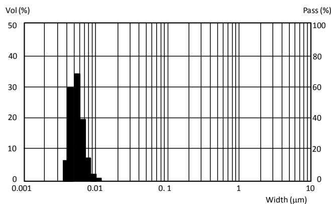
Figure S1. Dynamic light scattering (DLS) profile of alkyl-terminated Si NPs ( R_f = 0.1 ) column-separated by silica-gel column chromatography technique with gradient elution of dichloromethane-ethyl acetate.
