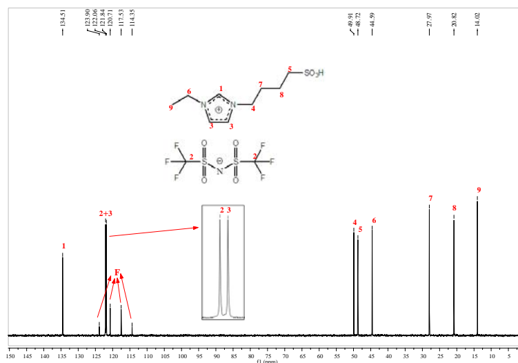
Fig. S3 13 C NMR spectrum of [EimC 4 SO 3 H] + NTf 2 -
