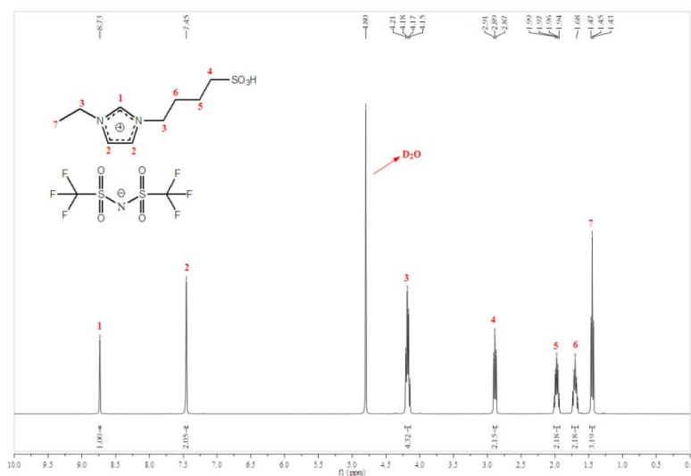
Fig. S4 1 H NMR spectrum of [EimC 4 SO 3 H] + NTf 2 -
