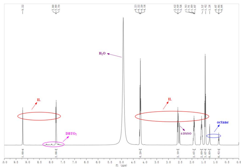
Fig. S6 1 H NMR spectrum of [EimC 4 SO 3 H]NTf 2 after extraction
