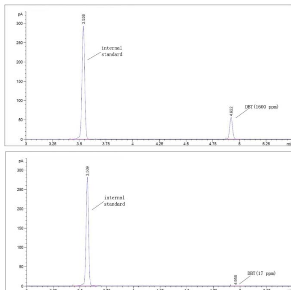
Fig. S5 The GC of DBT before extraction and after extraction
