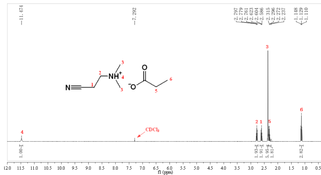
Fig.5 ^1\text{H} NMR spectrum of DMCEAP
