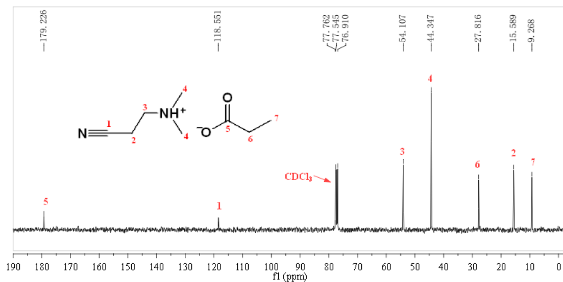
Fig.4 ^{13}\text{C} NMR spectrum of DMCEAP
