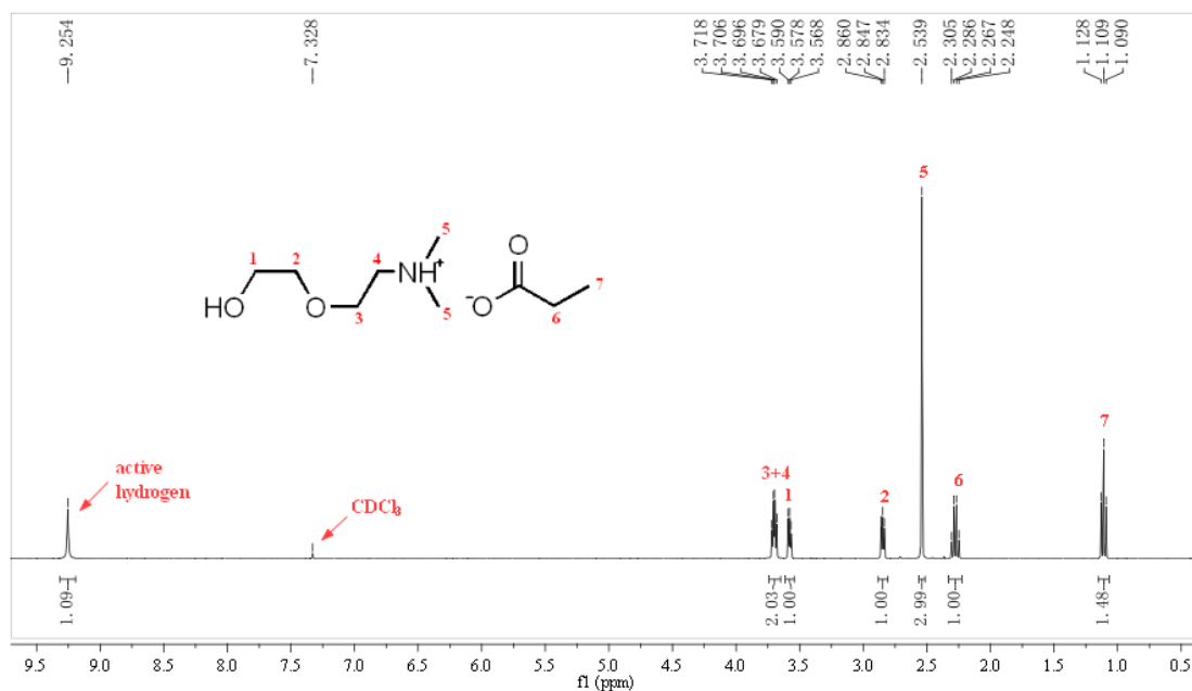
Fig.3 ^1\text{H} NMR spectrum of DMHEEAP
