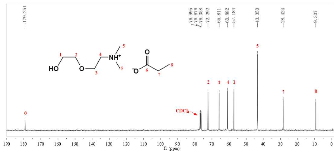
Fig.2 ^{13}\text{C} NMR spectrum of DMHEEAP
