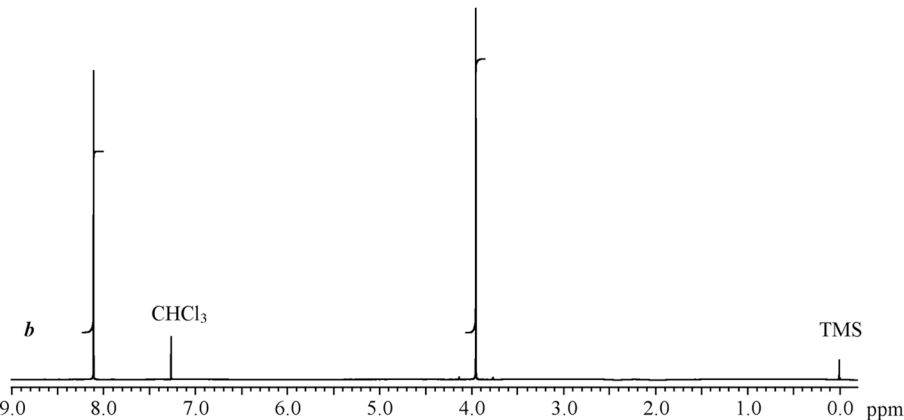
NMR spectra of DMT from limonene (a) and from non renewable resources (b)
