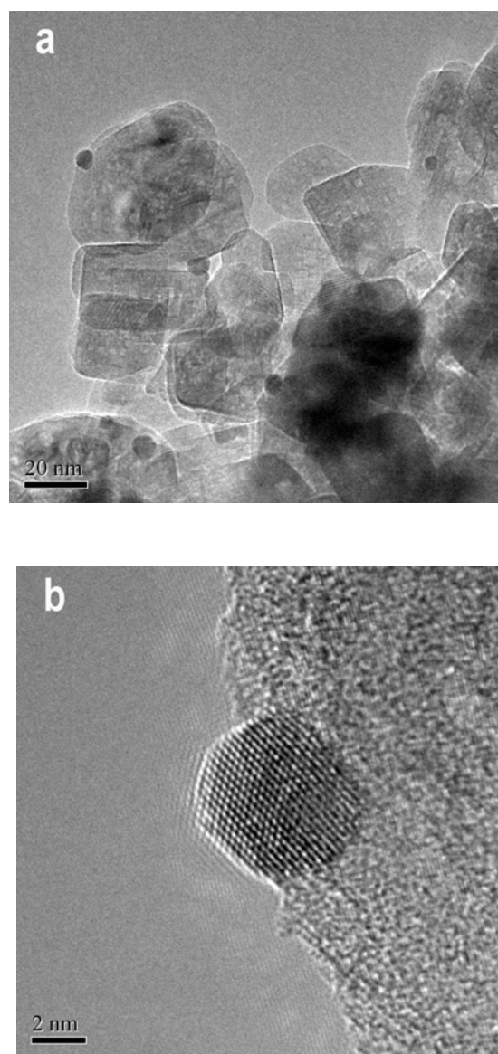
Figure S1. HRTEM image of the Pt 0.0002 -Au 0.005 /TiO 2 (a) and a selected metal particle (b).
