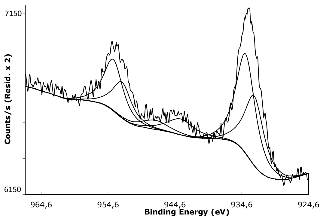
Figure 1. XPS Analysis of Cu@Fe NPs
