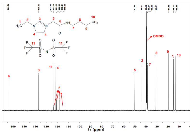
Fig.2 13 C NMR spectrum of [EimCH 2 CONHBu]NTf 2
