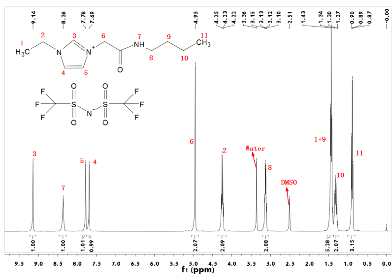
Fig.3 ^1\text{H} NMR spectrum of [\text{EimCH}_2\text{CONHBU}]\text{NTf}_2
