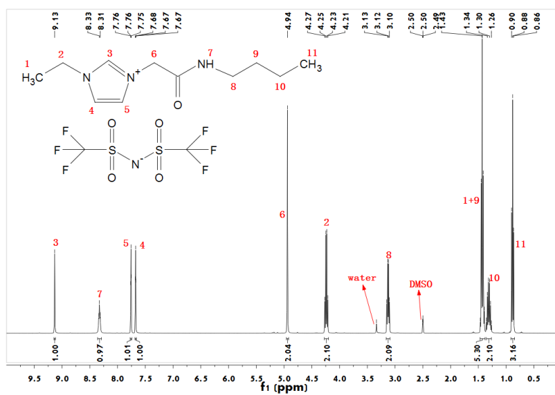
Fig.4 ^1\text{H} NMR spectrum of Recycled [\text{EimCH}_2\text{CONHBu}]\text{NTf}_2
