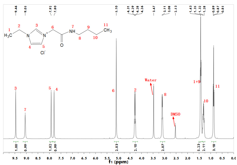
Fig.1 ^1\text{H} NMR spectrum of [\text{EimCH}_2\text{CONHBu}]\text{Cl}
