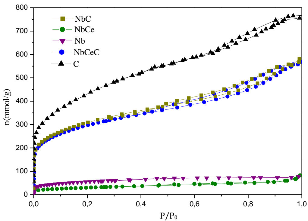
N 2 adsorption isotherms at 77 K on the different supports. Similar results were obtained after Pd impregnation
