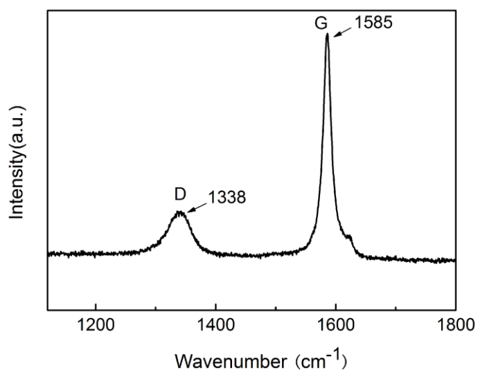
Figure 2S. The Raman spectrum of graphite
