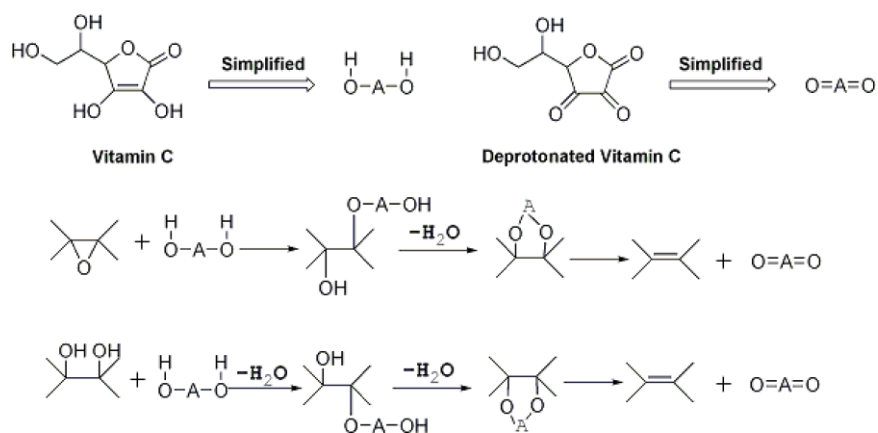
Scheme 1S. Schematic illustration of chemical reaction pathway of graphene oxide (GO) reduced by Vitamin C.
