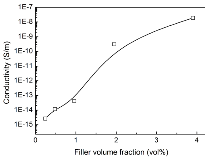
Figure 3S. The electrical conductivities of PS/t-RGO composites prepared by solution blending as a function of filler volume fraction.
