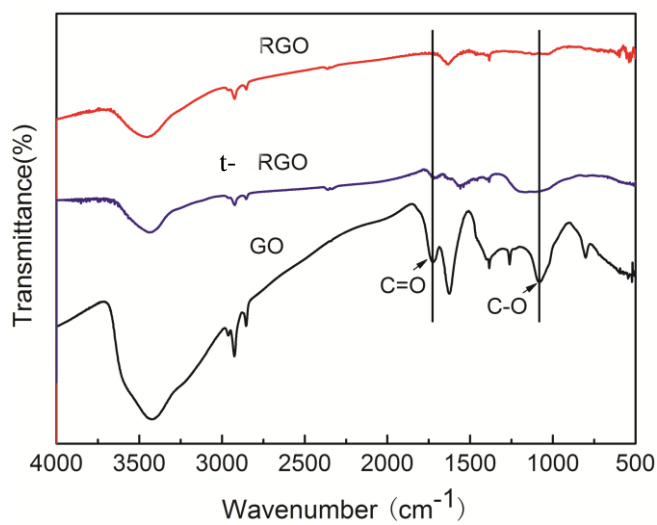
Figure 1S. FTIR spectra of GO, t-RGO, and RGO.
