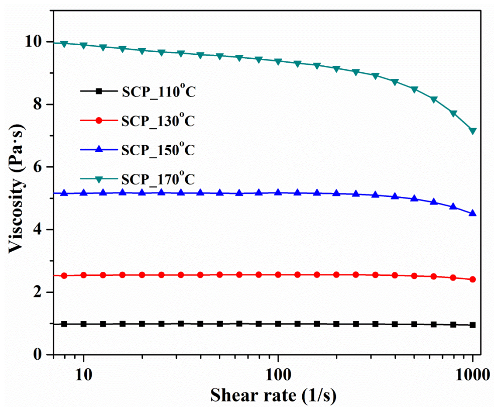
Fig. 7 Rheological behavior of polyols prepared at different reaction temperatures
