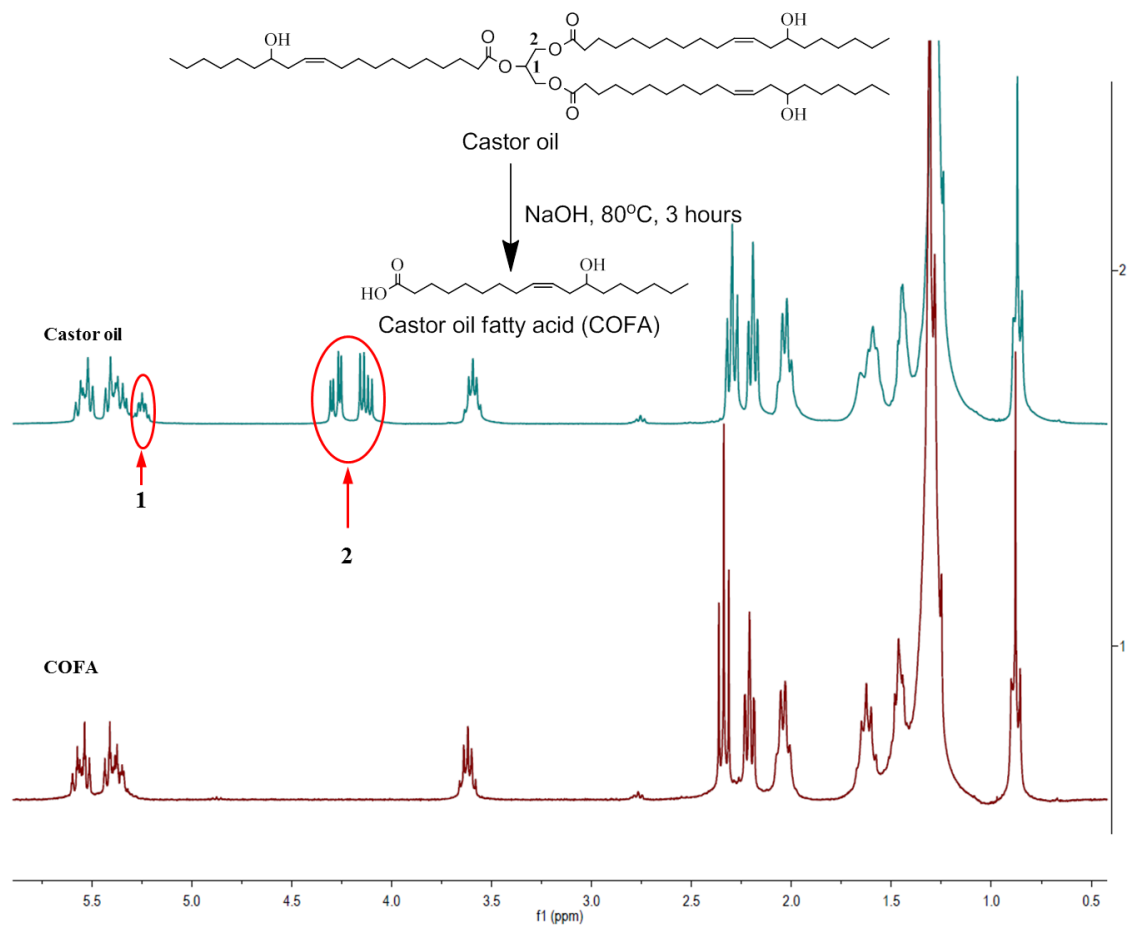
Fig. 1 1 H-NMR spectra of CO and COFA
