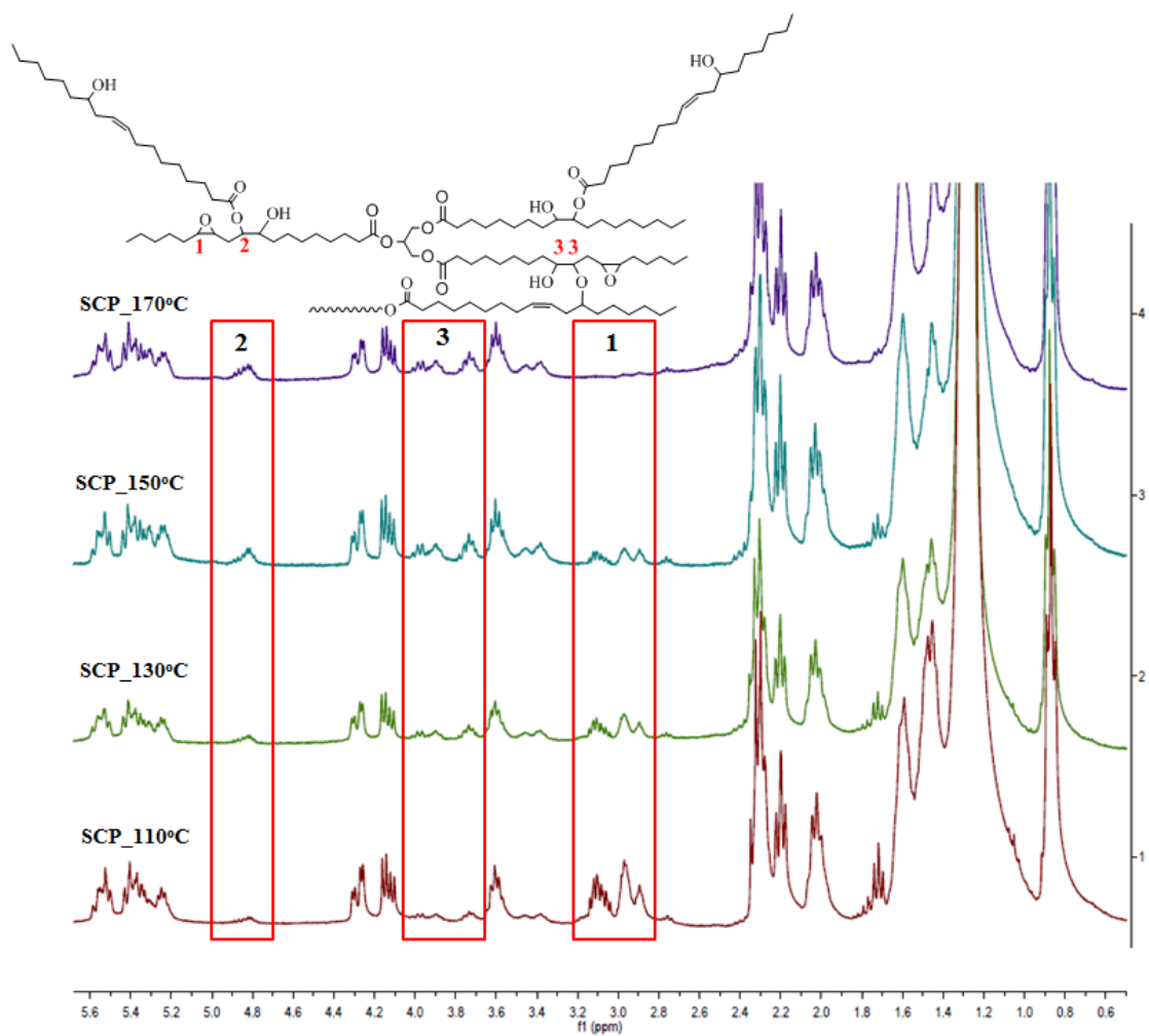
Fig. 2 1 H-NMR spectra of SCP for different reaction temperatures
