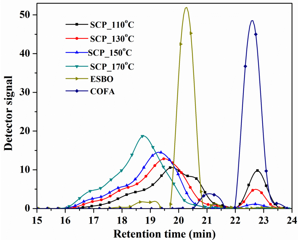
Fig. 5 GPC curves of SCP for different reaction temperatures
