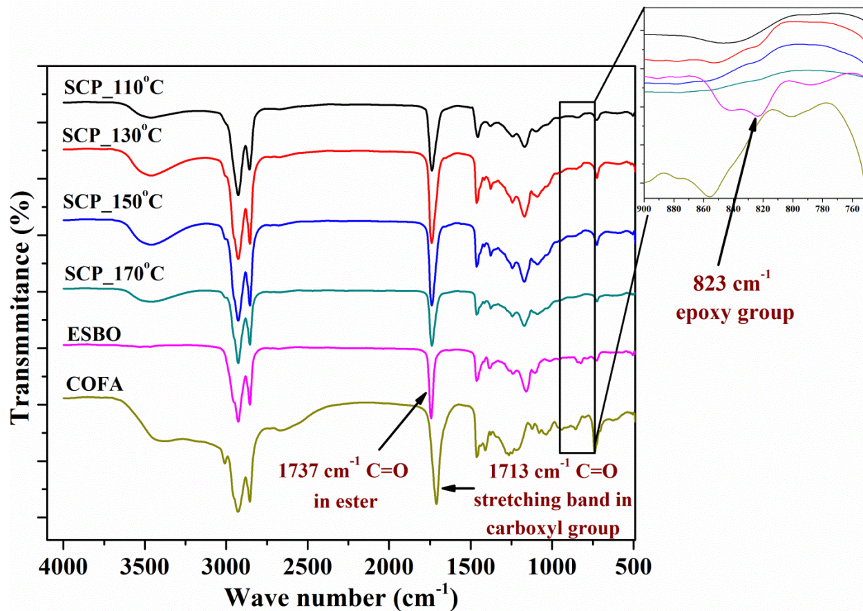
Fig. 3 FTIR spectra of SCP for different reaction temperatures
