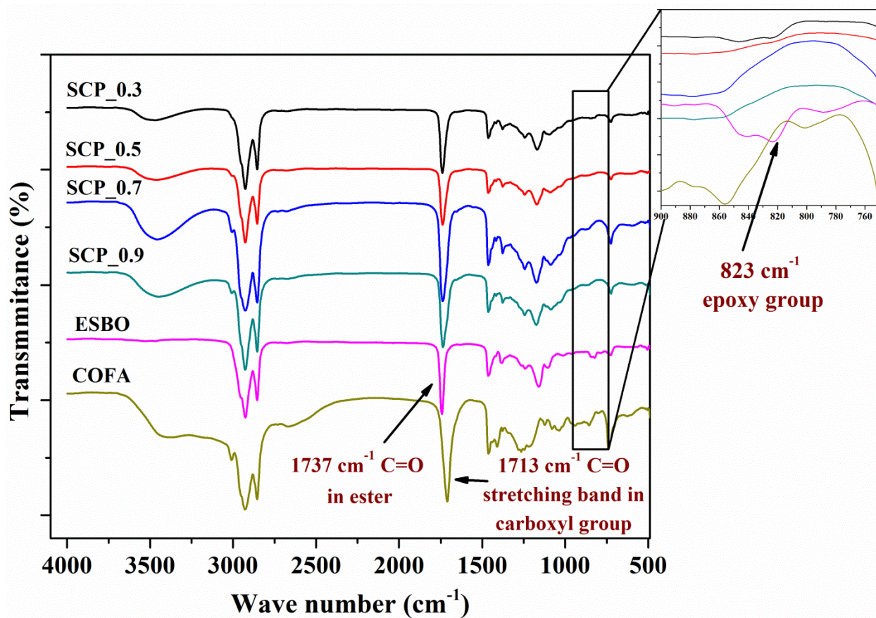
Fig. 4 FTIR spectra of SCP for different reaction ratios of carboxyl to epoxy groups
